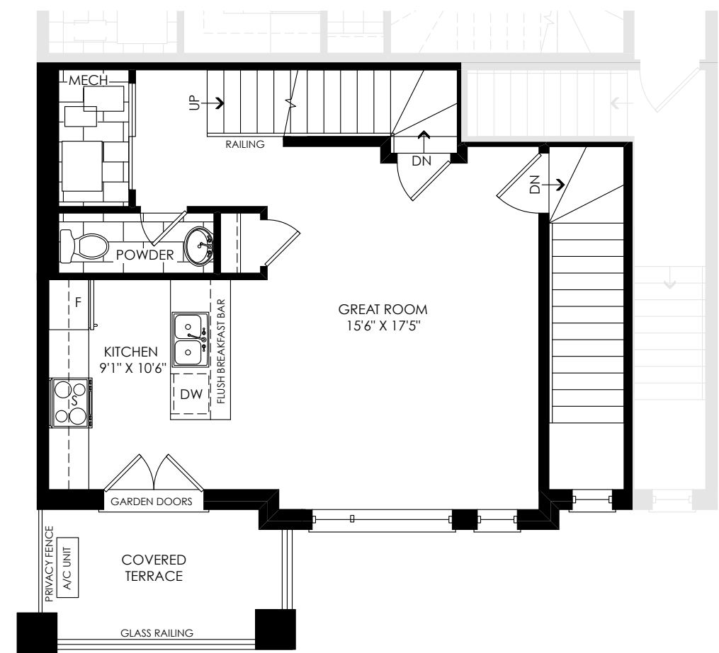
INTERIOR SECOND FLOOR PLAN (FRONT)
