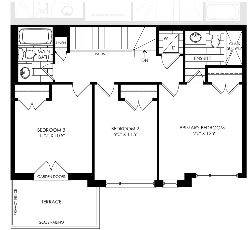
INTERIOR THIRD FLOOR PLAN (FRONT)
