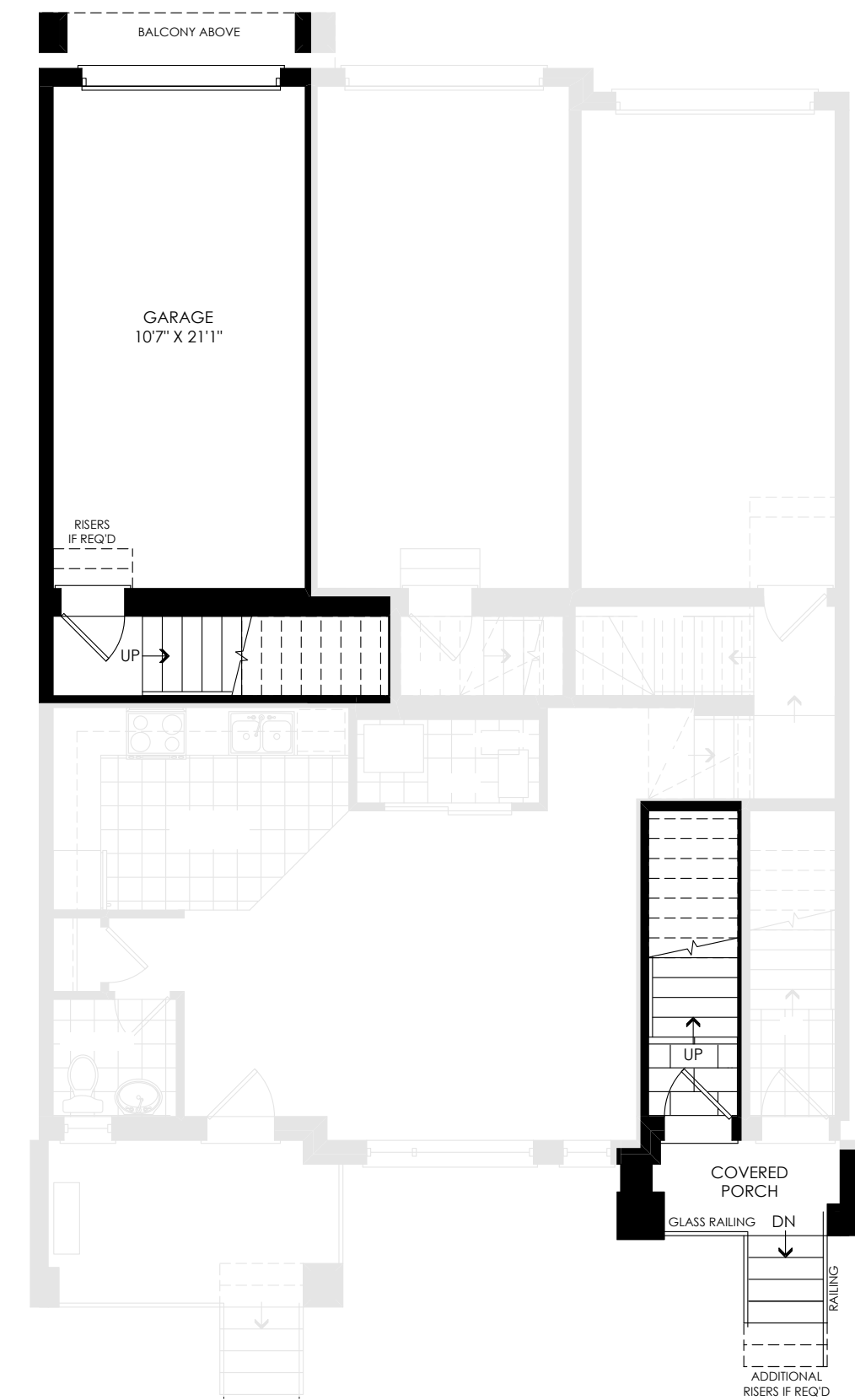
INTERIOR MAIN FLOOR PLAN (FRONT)
