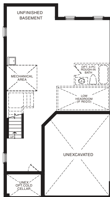
BASEMENT PLAN STYLE A
