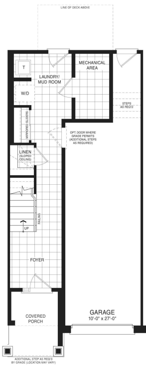
GROUND FLOOR PLAN STYLE A1
