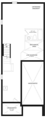
BASEMENT PLAN STYLE A
