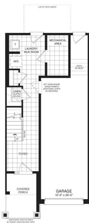
GROUND FLOOR PLAN STYLE A1
