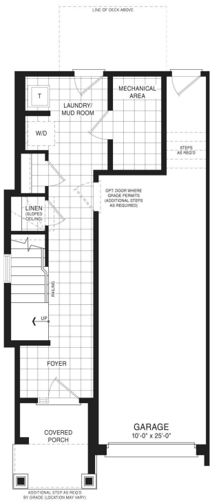
GROUND FLOOR PLAN STYLE A1
