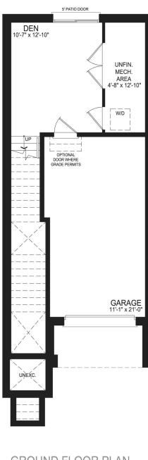
GROUND FLOOR PLAN STYLE A1
