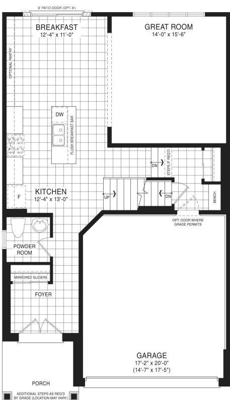
MAIN FLOOR PLAN STYLE A
