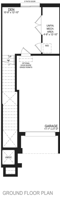
GROUND FLOOR PLAN STYLE A1
