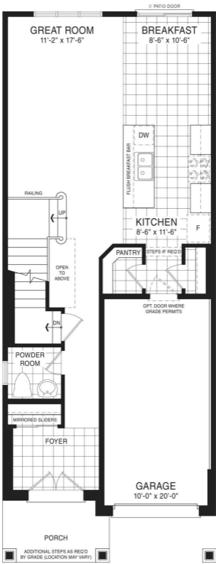
MAIN FLOOR PLAN STYLE A
