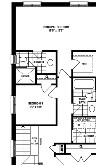
PARTIAL OPT. SECOND FLOOR ELEV. 'B' 4 BEDROOM END UNIT
