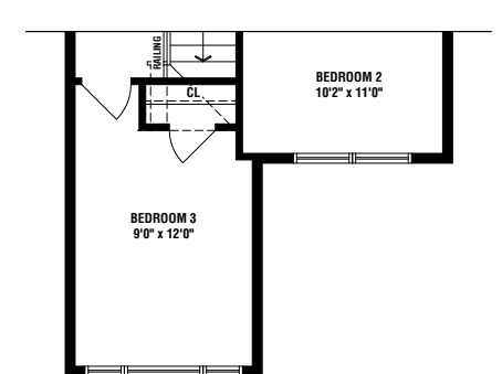
PARTIAL SECOND FLOOR ELEV. 'B'
