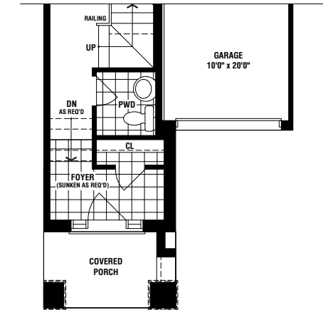
PARTIAL GROUND FLOOR ELEV. 'B'
