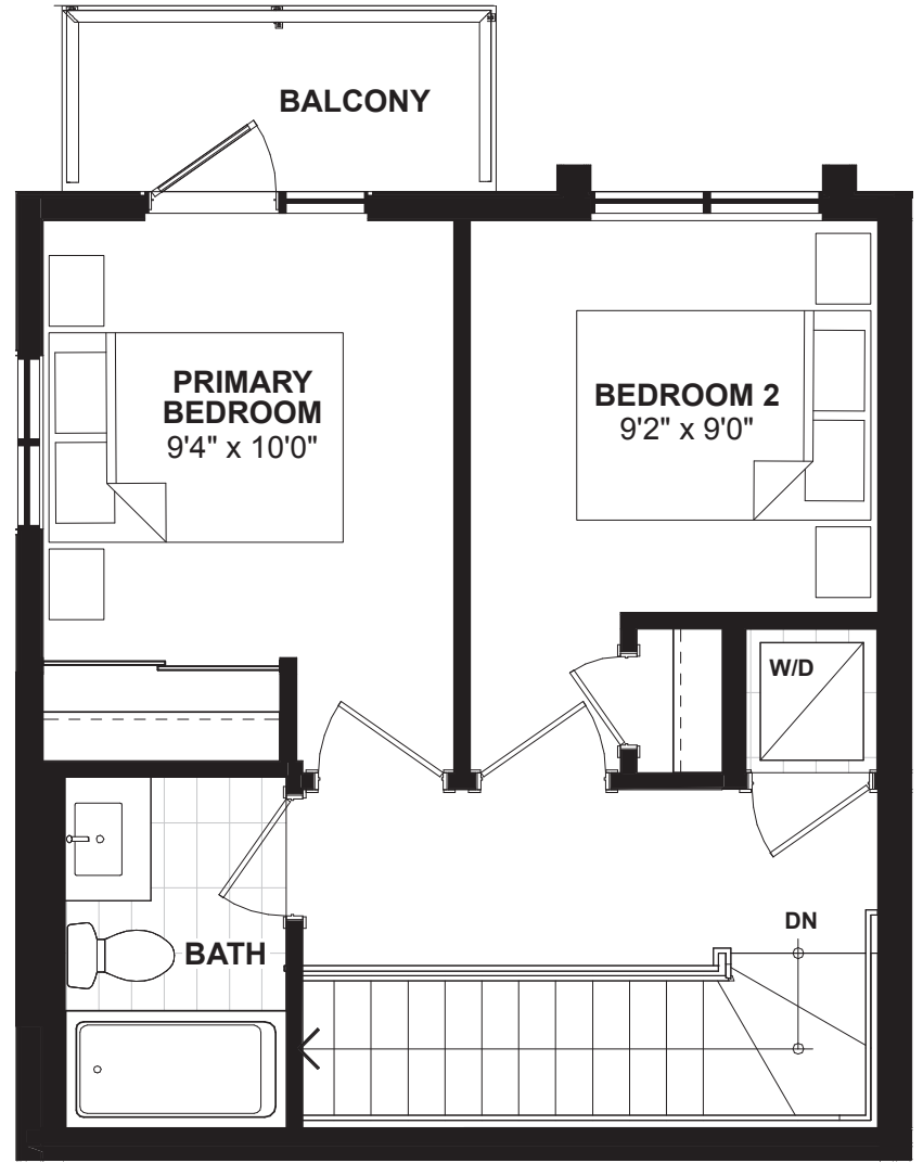
TH LEVEL 3
