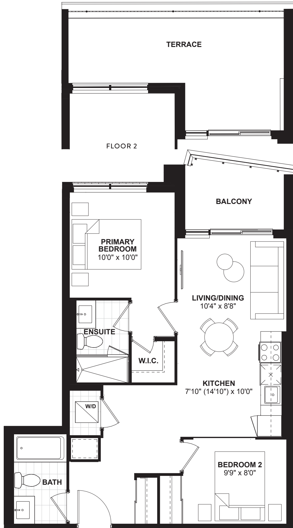
FLOORS 3-6
