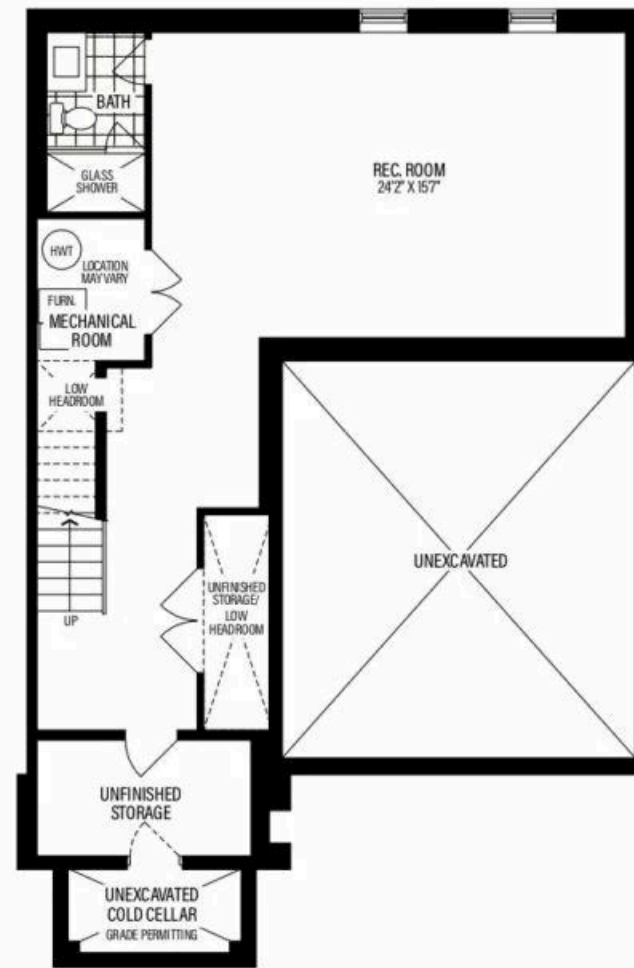
Lower Level ELEV 'A'
