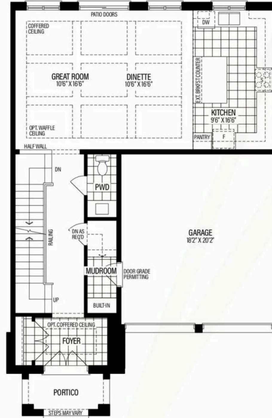
Main Level ELEV A
