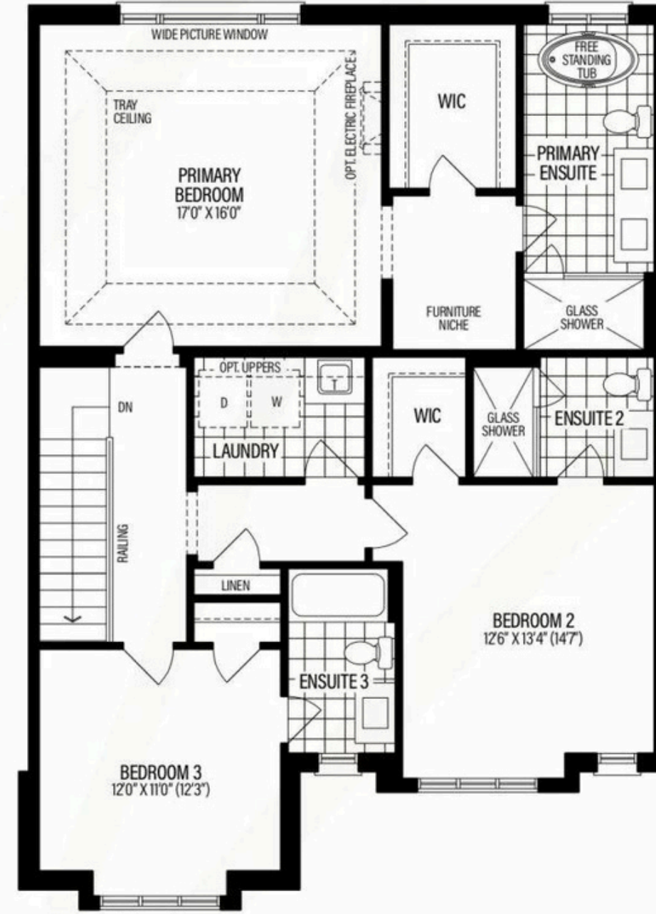
Second Level ELEV A
