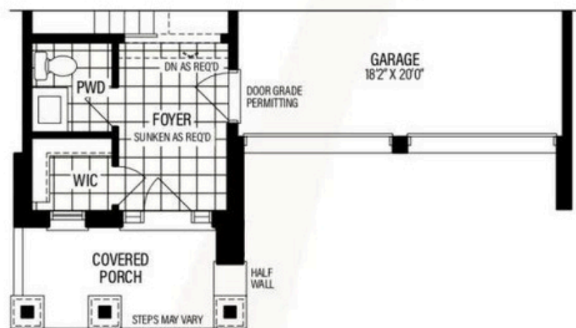
Part Main Level ELEV 'B'
