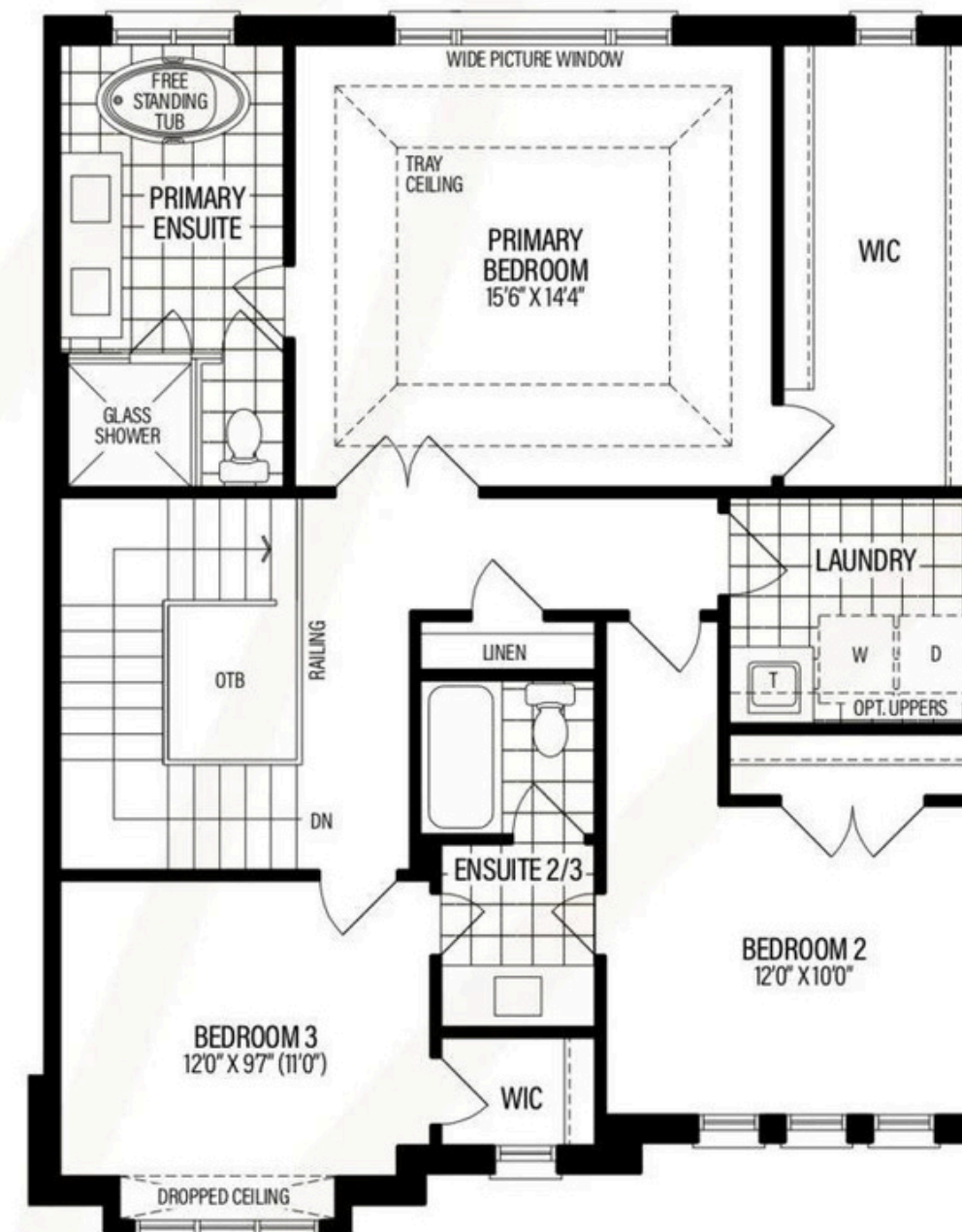
Second Level ELEV 'A'
