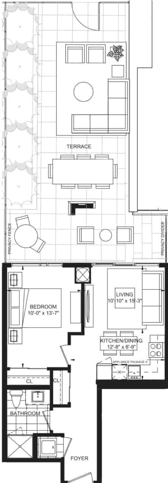
1ST FL - UNIT #20
