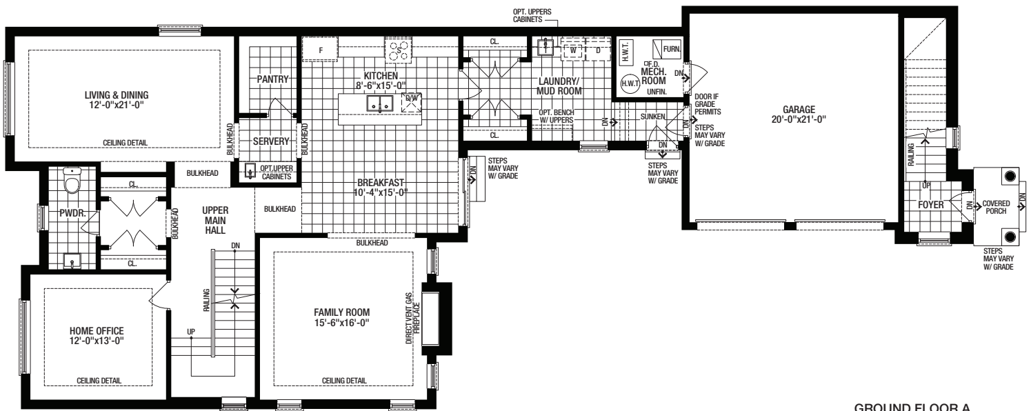
GROUND FLOOR A
