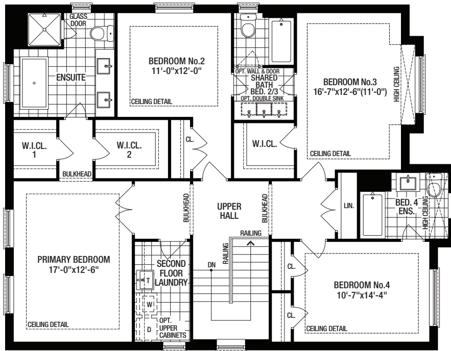
SECOND FLOOR A
