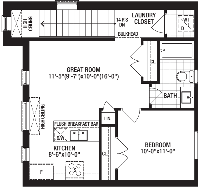
SECOND FLOOR A COACH HOUSE
