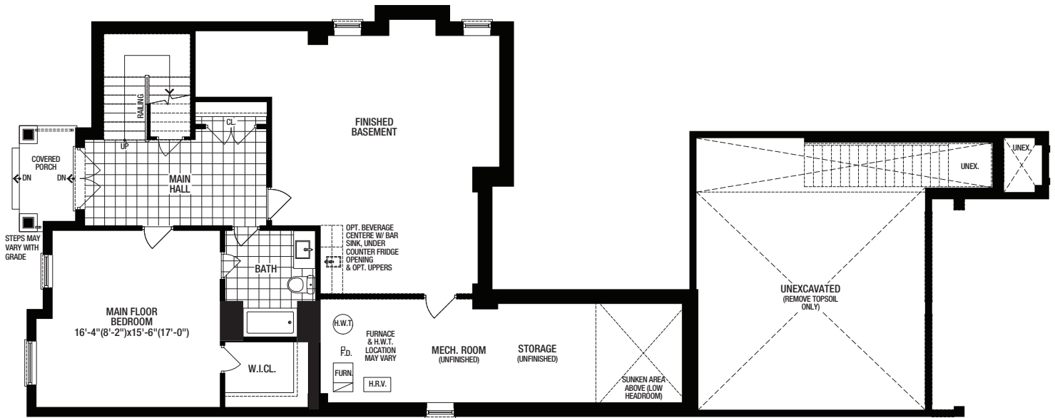
OPTIONAL FINISHED BASEMENT FLOOR A
