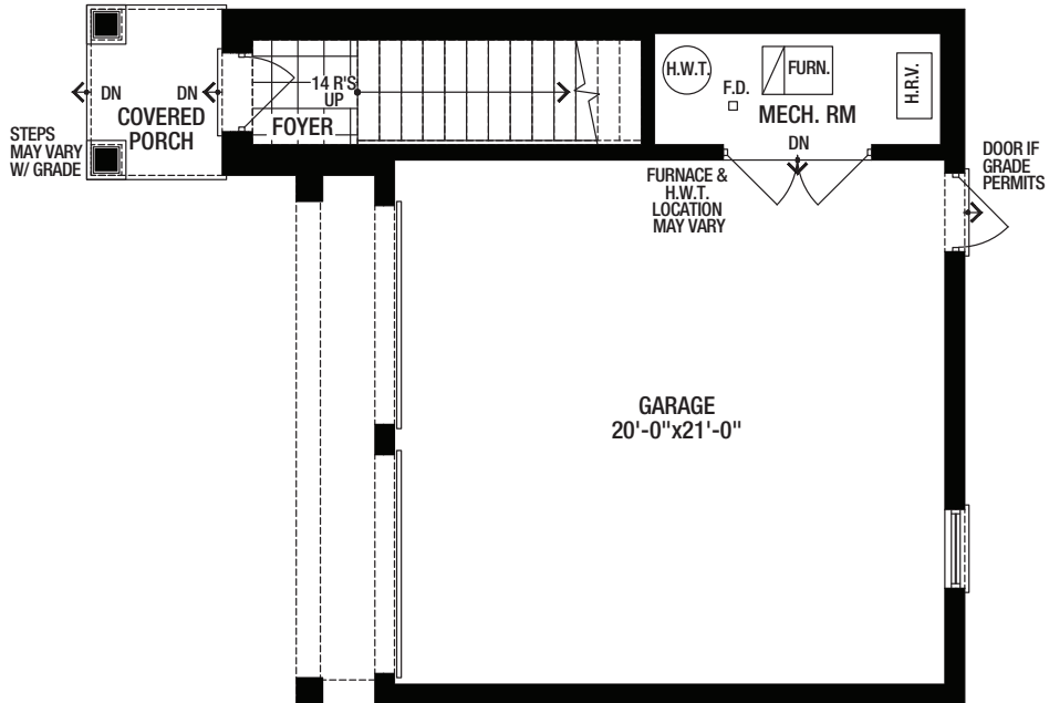
GARAGE A
