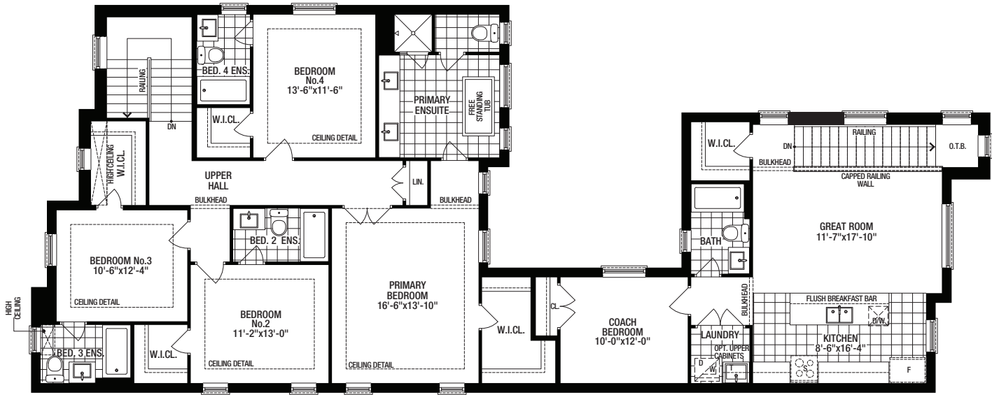
SECOND FLOOR A
