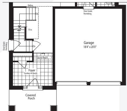
First Floor Elevation C
