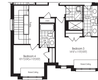
Opt. 5 Bedroom Second Floor Elevation B
