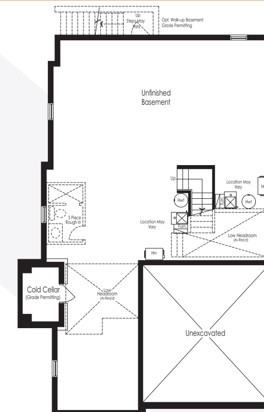
Basement - Elevation B
