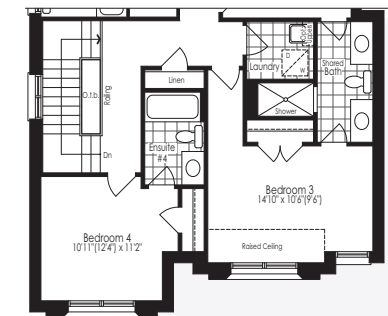
Opt. 5 Bedroom Second Floor Elevation C
