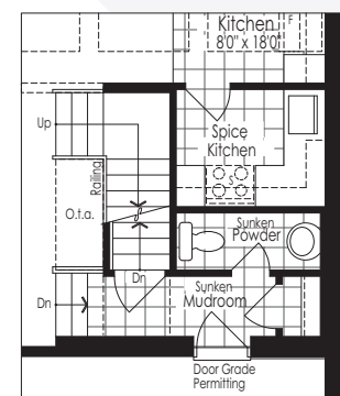
Optional First Floor With Spice Kitchen
