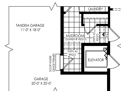
Partial Opt. Ground Floor with Elevator Elevation A & B
