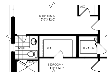
Partial Opt. Second Floor with Elevator Elevation A & B
