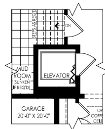
Partial Ground Floor with Elevator Elevation A & B
