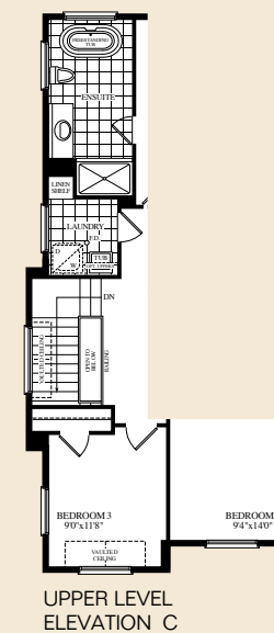
OPT. UPPER LEVEL W/3 BATHROOMS ELEVATION C
