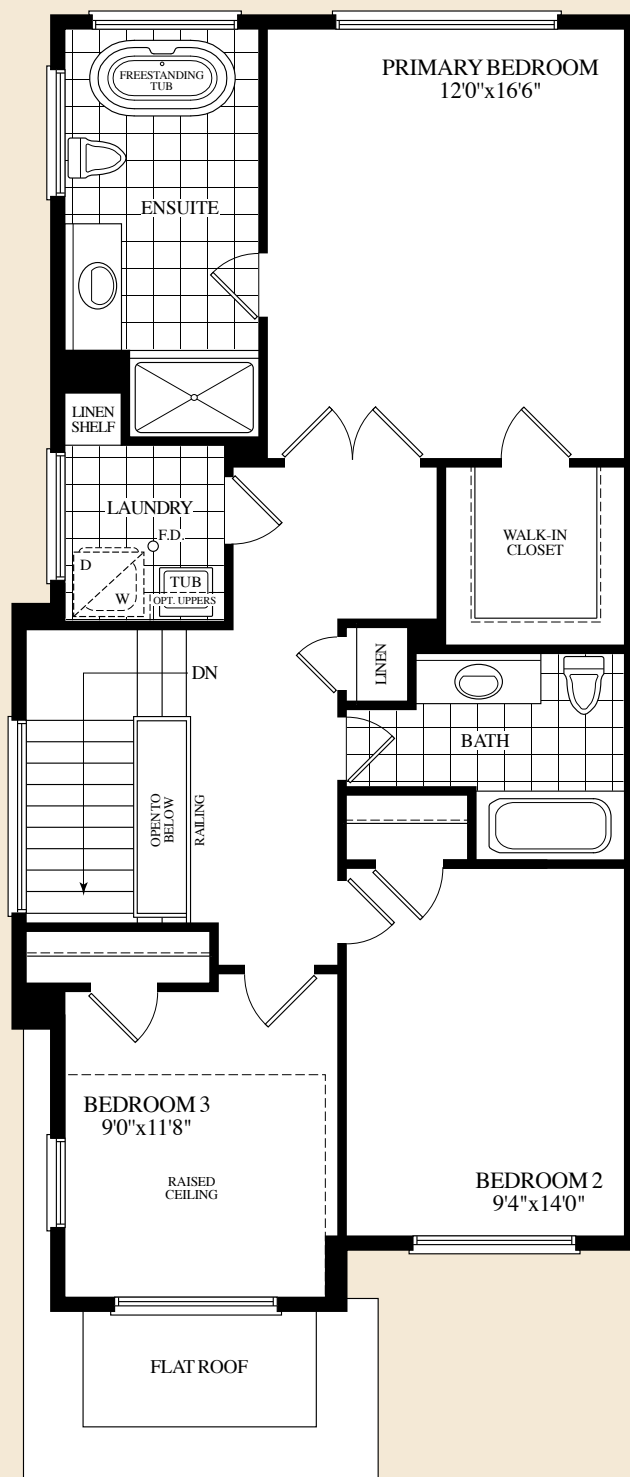
UPPER LEVEL ELEVATION A
