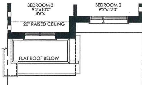
OPT. SECOND FLOOR PLAN, EL. 'B' W/ FLEX SPACE
