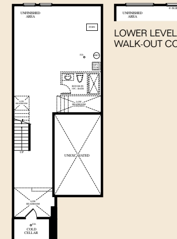
LOWER LEVEL ELEVATION A, B & C
