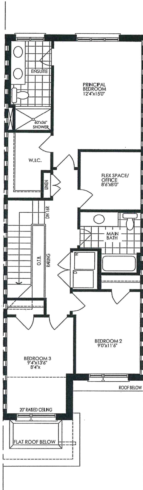
OPT. SECOND FLOOR PLAN, EL. 'A' W/ FLEX SPACE (EL. 'B' & 'C' SIMILAR)
