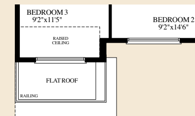
OPT. UPPER LEVEL W/3 BATHROOMS ELEVATION B
