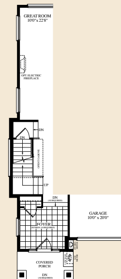
MAIN LEVEL ELEVATION B
