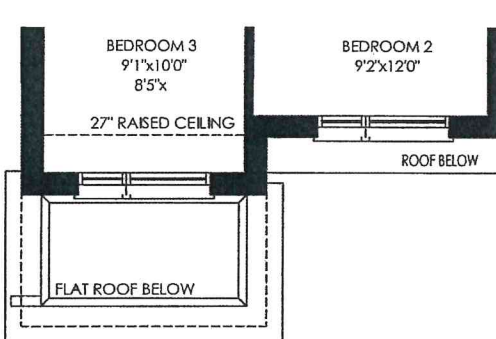
SECOND FLOOR PLAN, EL. 'B'
