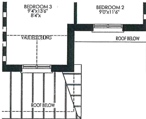
OPT. SECOND FLOOR PLAN, EL. 'C' W/ FLEX SPACE
