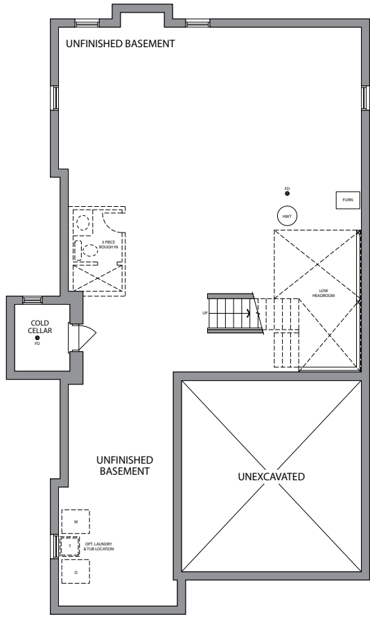
BASEMENT ELEV. A
