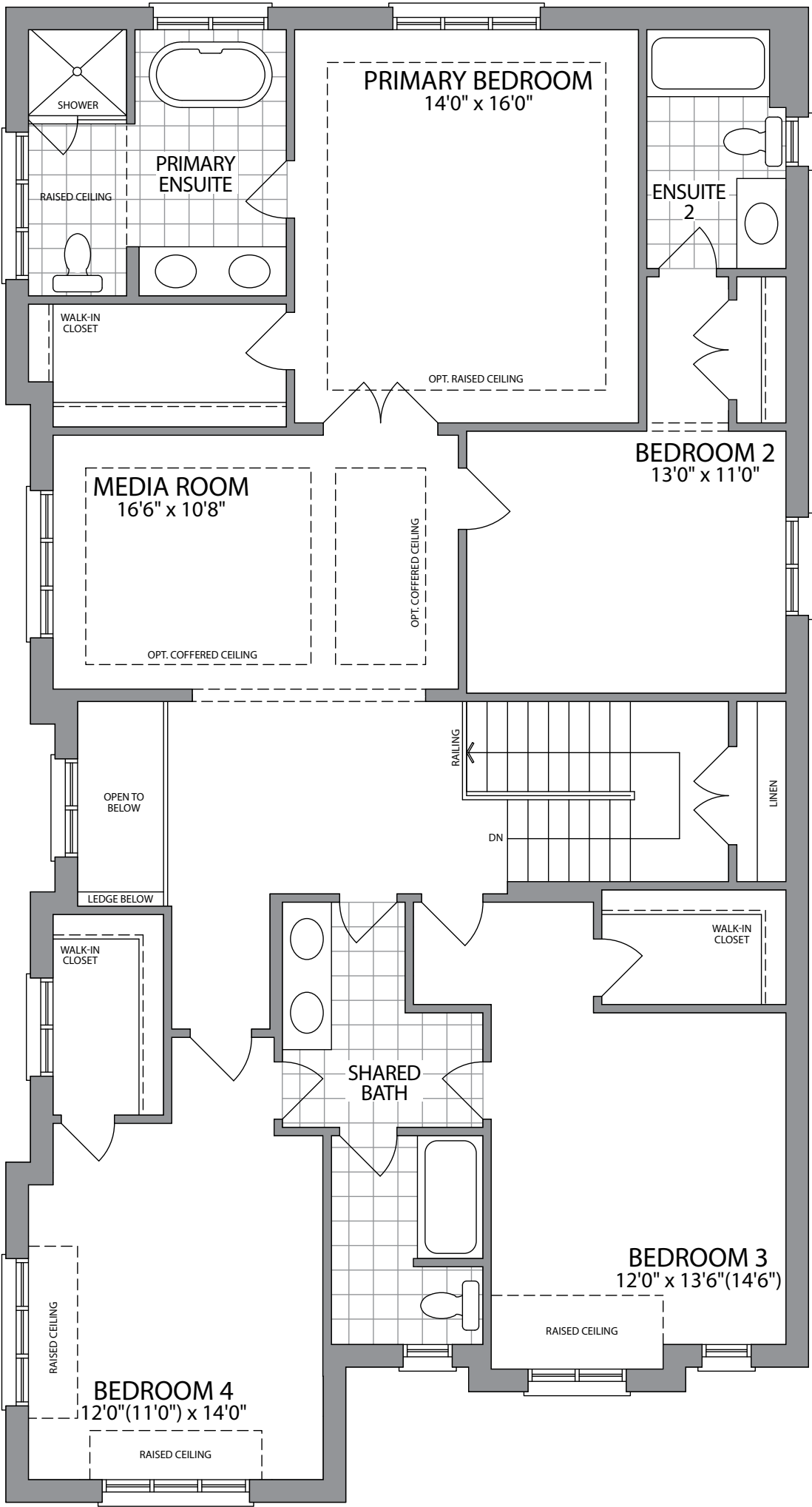
SECOND FLOOR ELEV. A
