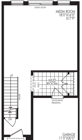
PART, OPT. FIRST FLOOR W/ MEDIA ROOM PLAN EL. 'A' (ELEV. 'B' SIMILAR)
