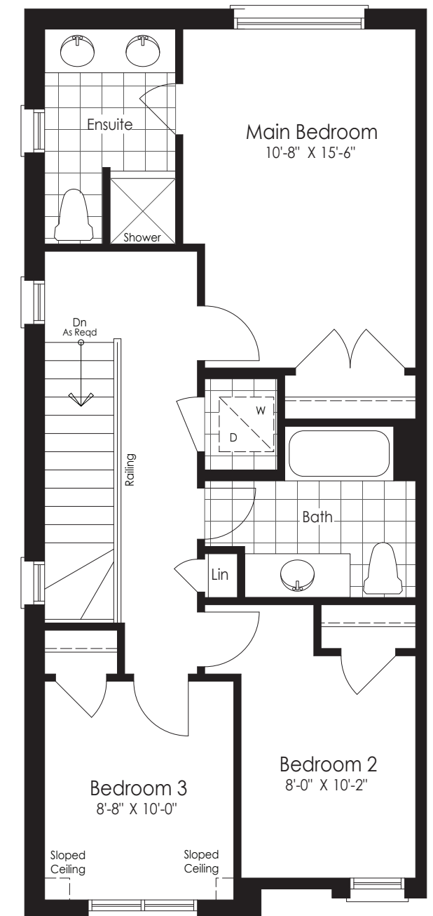
Alt. Upper Floor Elevation A
