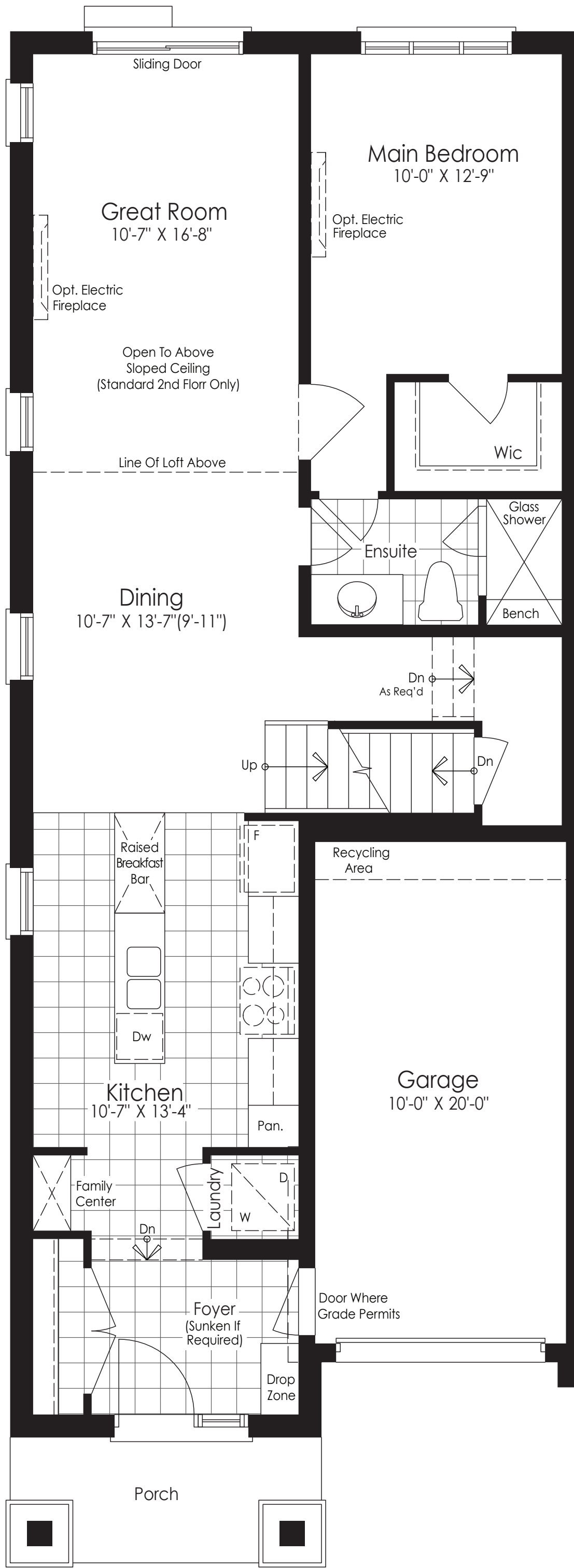
Main Floor Elevation A1, A2 & B
