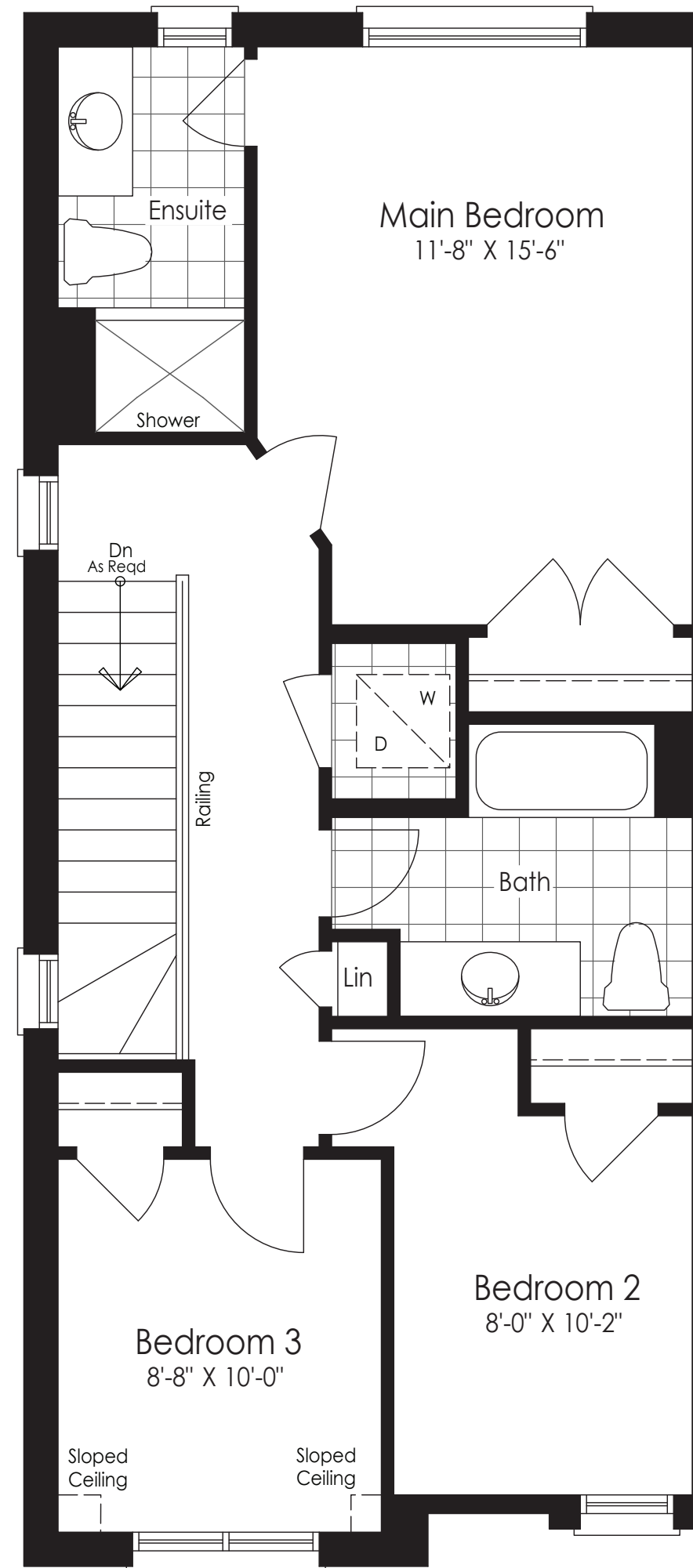
Upper Floor Elevation A
