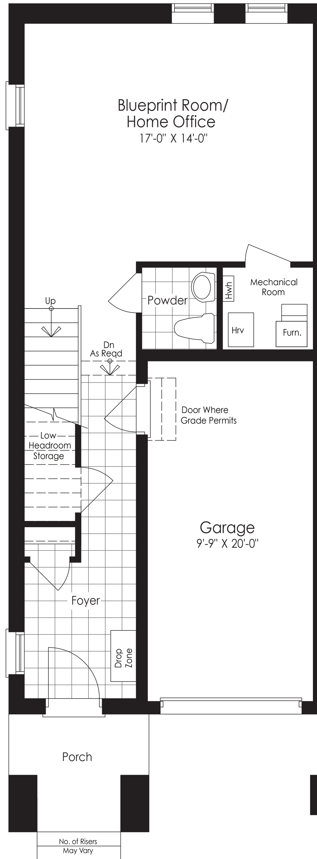
Ground Floor Elevation A, B1, C & D
