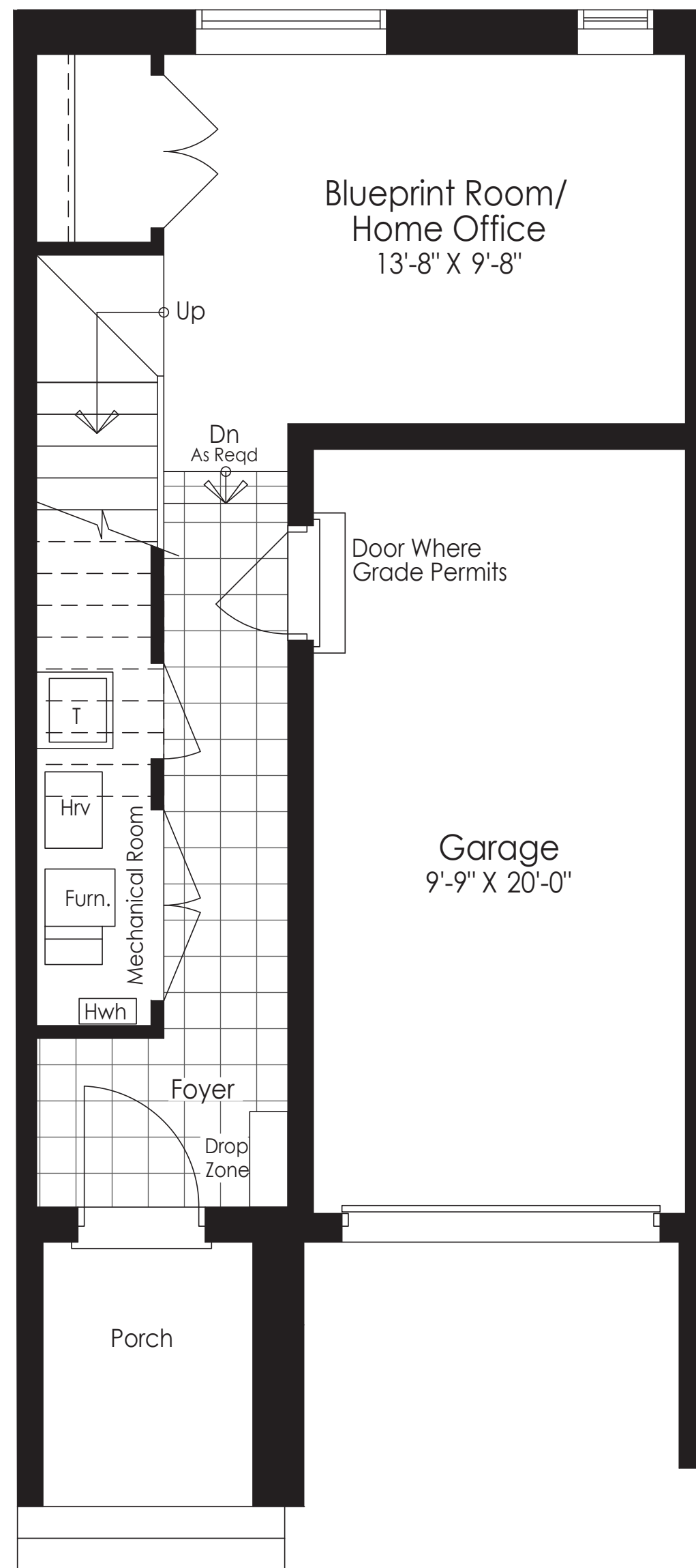
Ground Floor Elevation A & B
