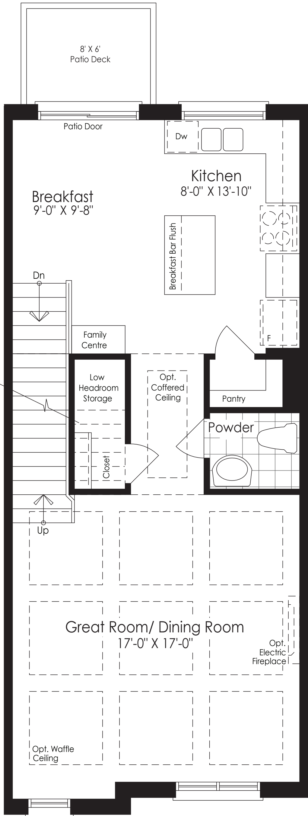
Main Floor Elevation A
