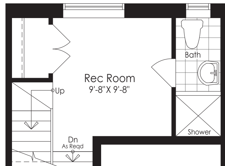
Ground Floor with Opt. Full Bath Elevation A & B
