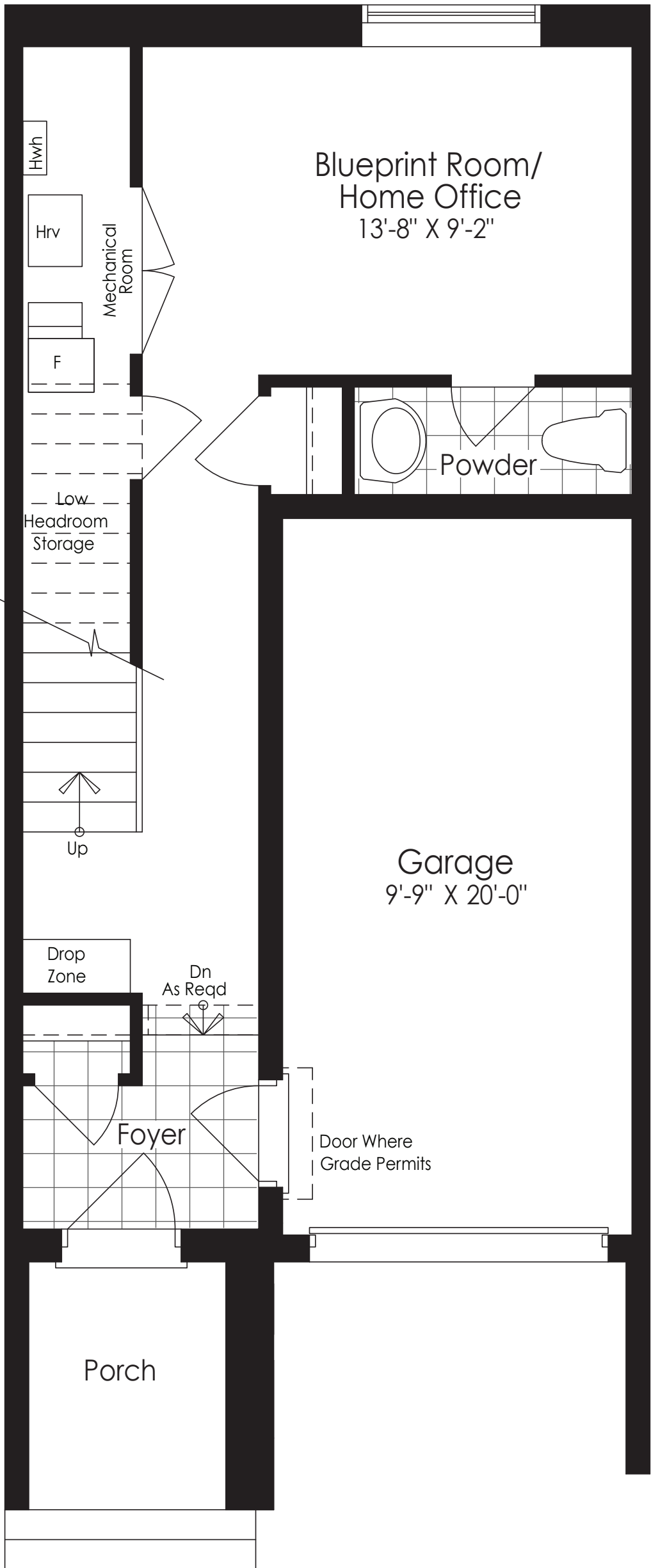
Ground Floor Elevation A & B
