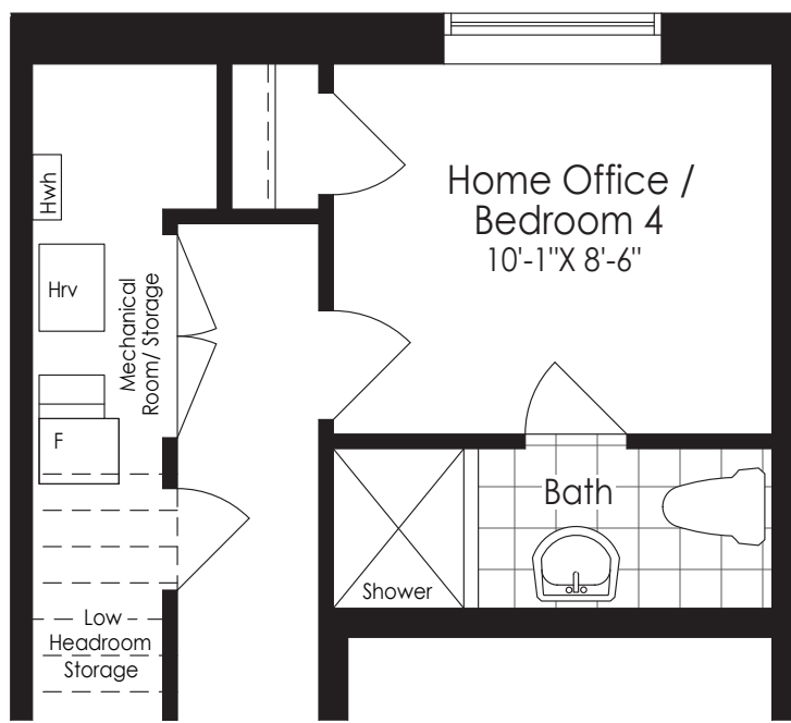
Ground Floor with Opt. Office/Bedroom & Bath Elevation A & B
