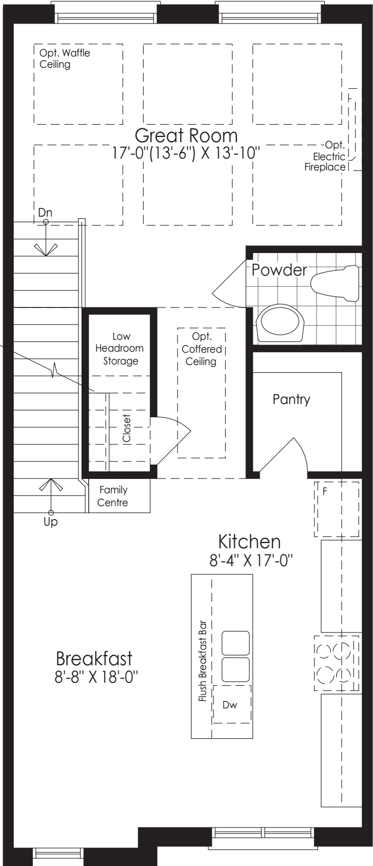
Alt. Main Floor Elevation A
