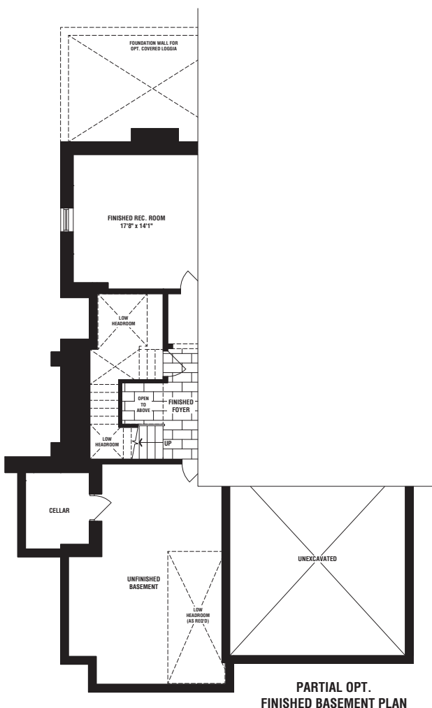
PARTIAL OPT. FINISHED BASEMENT PLAN ELEV. 'B'
