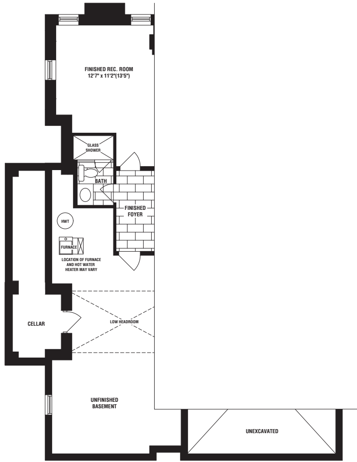
PARTIAL OPT. FINISHED BASEMENT PLAN ELEV. 'C'
