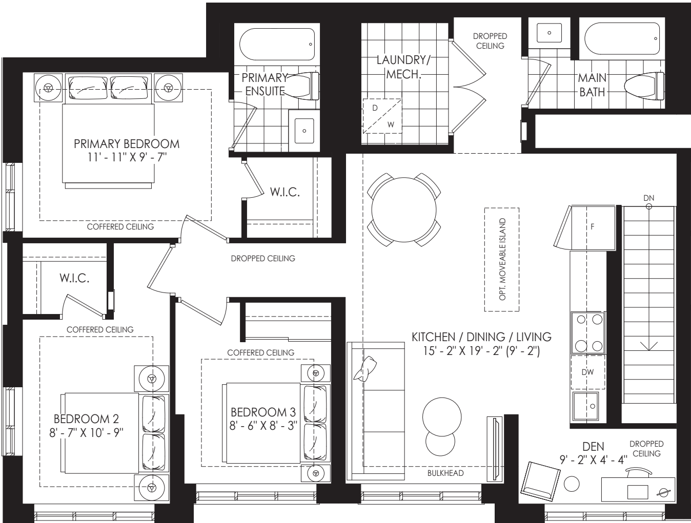
SECOND FLOOR (8 FEET CEILING)
