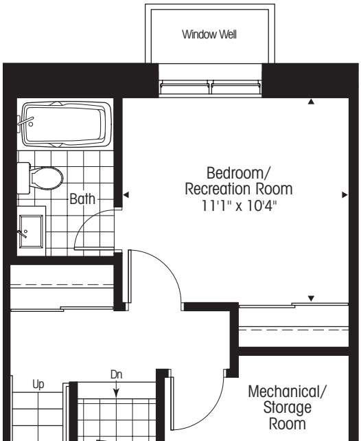
**OPTIONAL UPGRADED LAYOUT Lower Level Floor-353 SF
