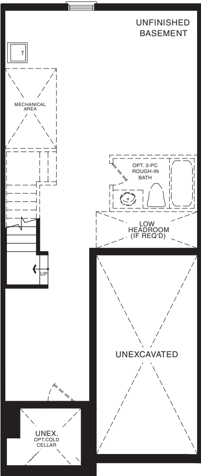
BASEMENT PLAN STYLE A1
