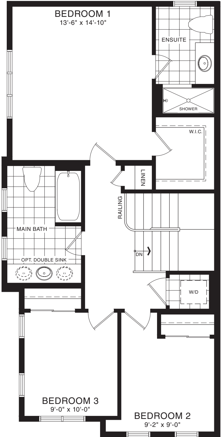
SECOND FLOOR PLAN STYLE A1
