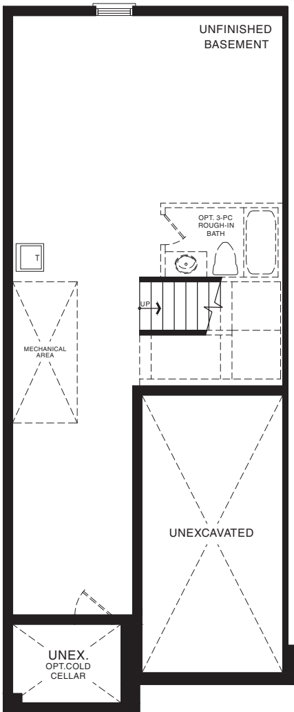
BASEMENT PLAN STYLE A1
