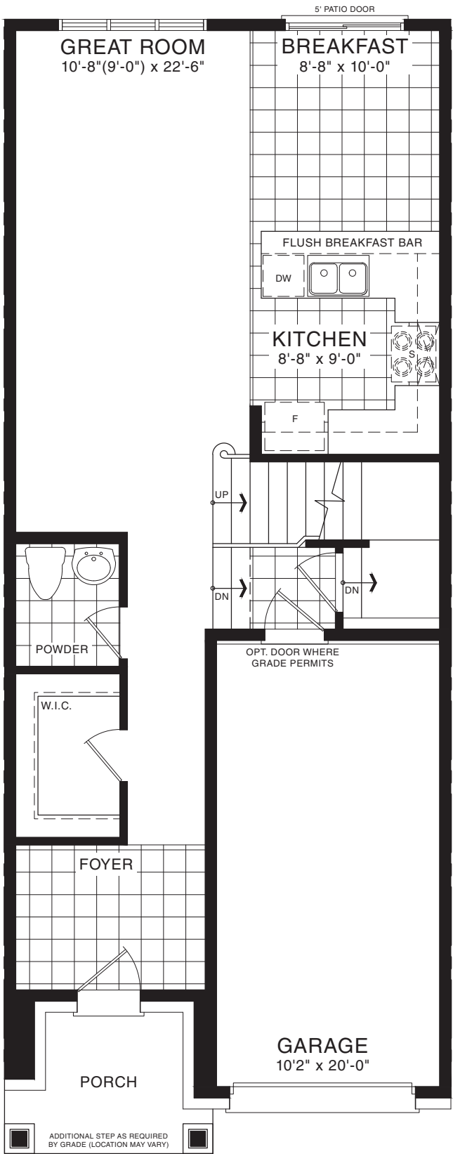
MAIN FLOOR PLAN STYLE A1
