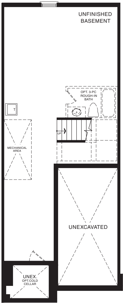
BASEMENT PLAN STYLE A1
