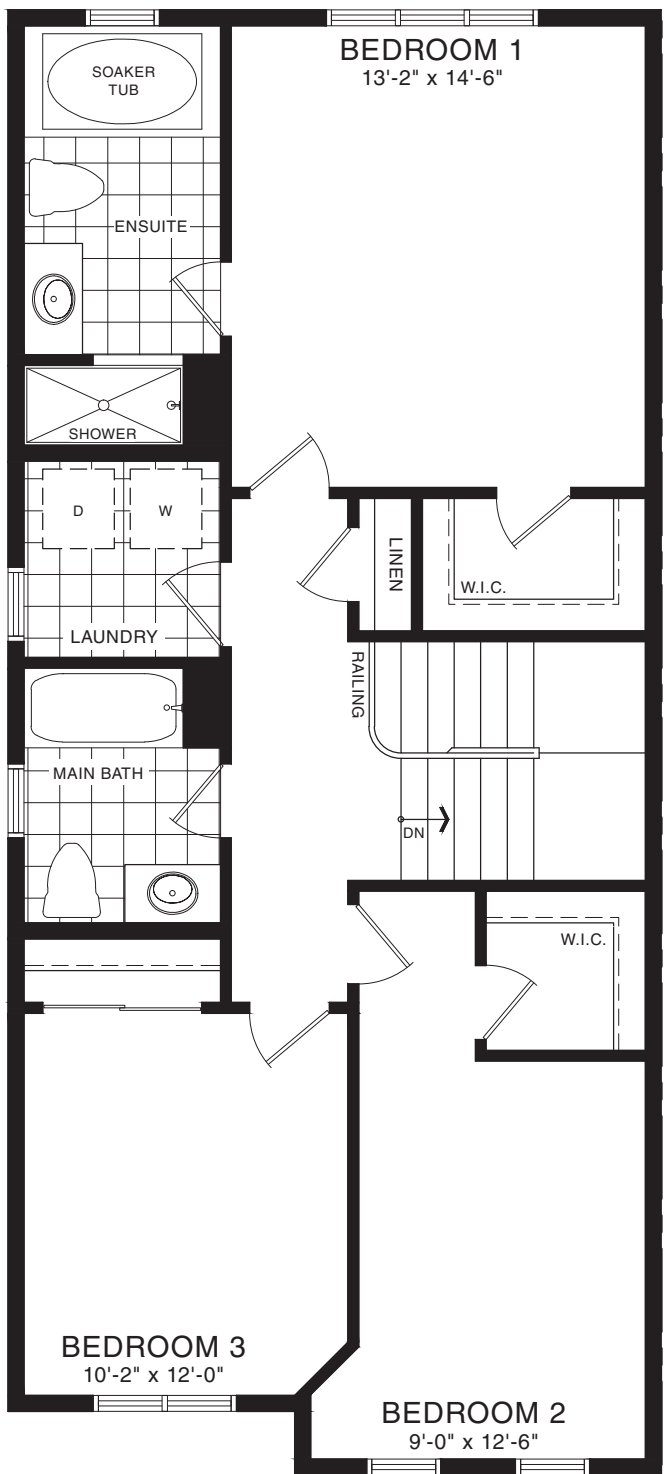
SECOND FLOOR PLAN STYLE A1
