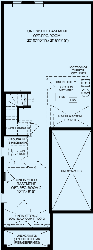
BASEMENT | ELEVATION A, B +C
