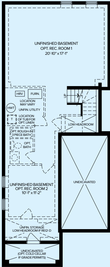
BASEMENT | ELEVATION A, B + C
