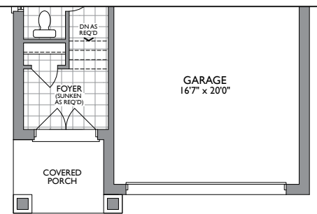
PARTIAL MAIN LEVEL ELEV. B & C
