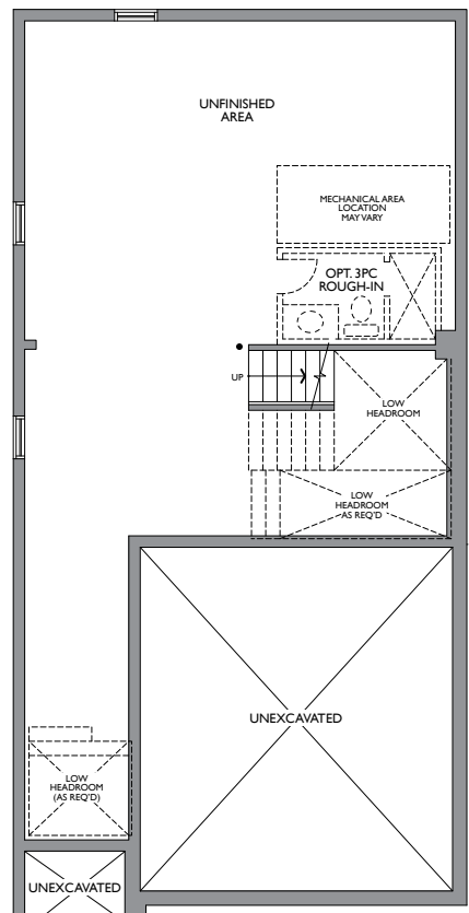
LOWER LEVEL ELEV. A & B
