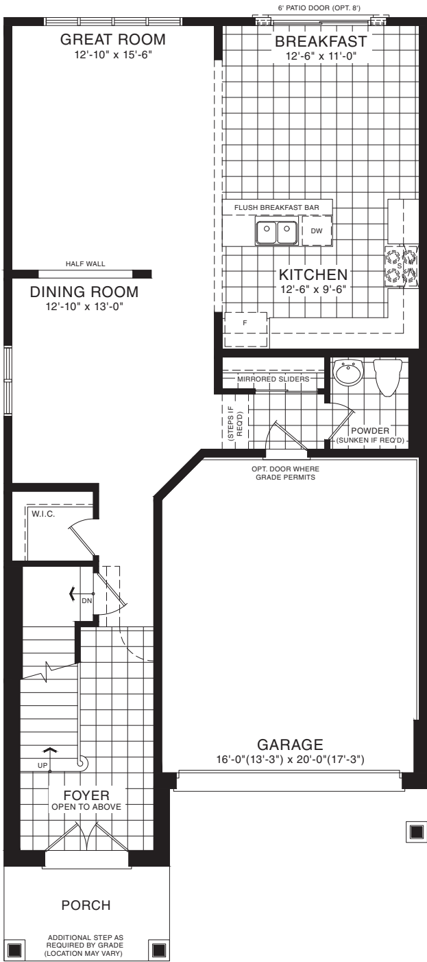
MAIN FLOOR PLAN ELEVATION A
