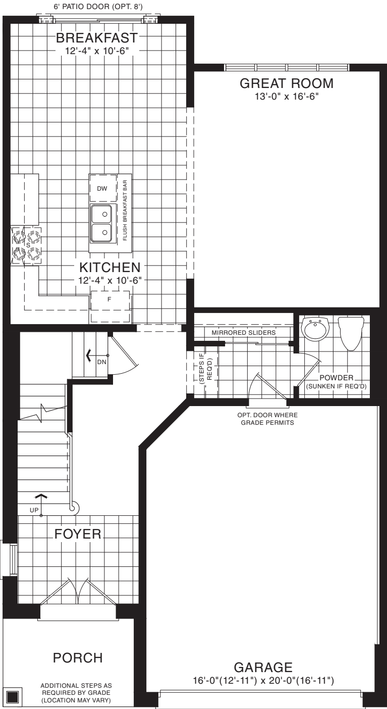
MAIN FLOOR PLAN ELEVATION A
