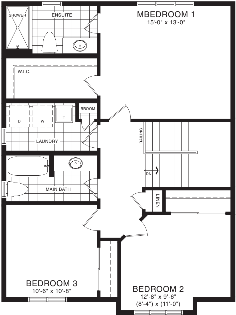
SECOND FLOOR PLAN ELEVATION A
