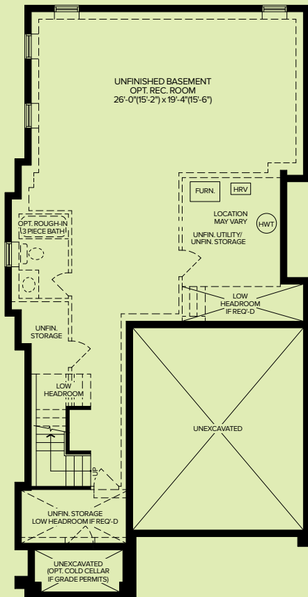
BASEMENT | ELEVATION C
