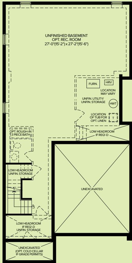
BASEMENT | ELEVATION A, B + C
