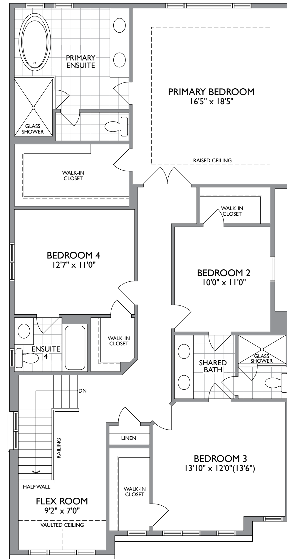
UPPER LEVEL ELEV. A
