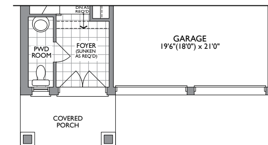
PARTIAL MAIN LEVEL ELEV. B
