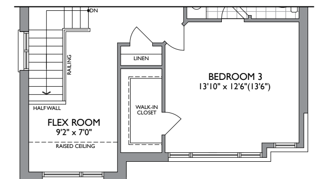
PARTIAL LEVEL ELEV. C
