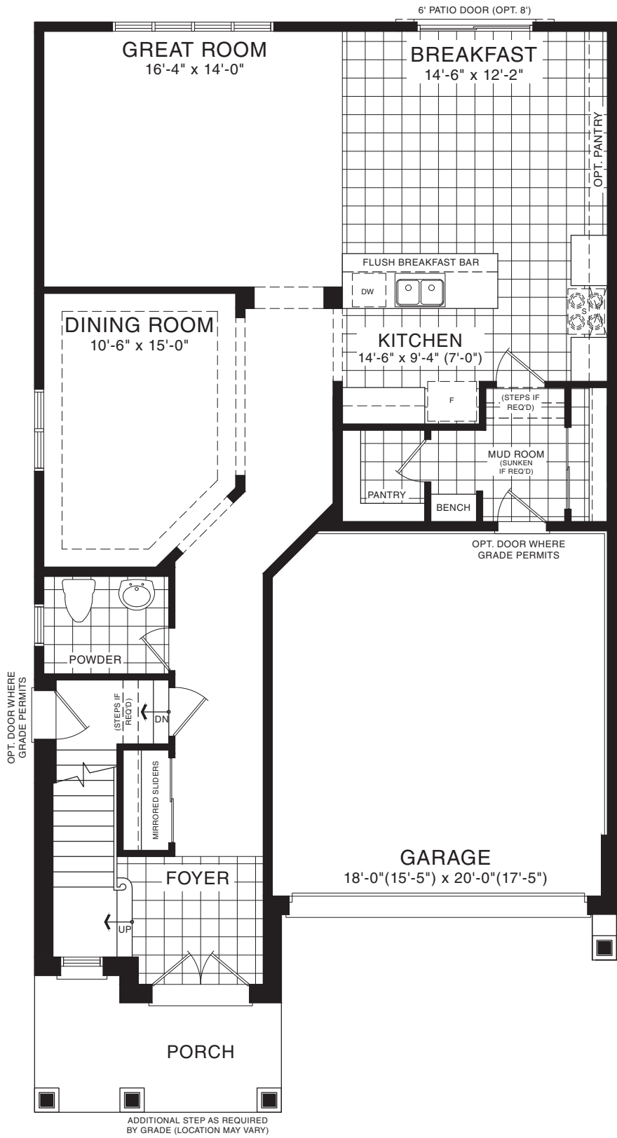
MAIN FLOOR PLAN STYLE A
