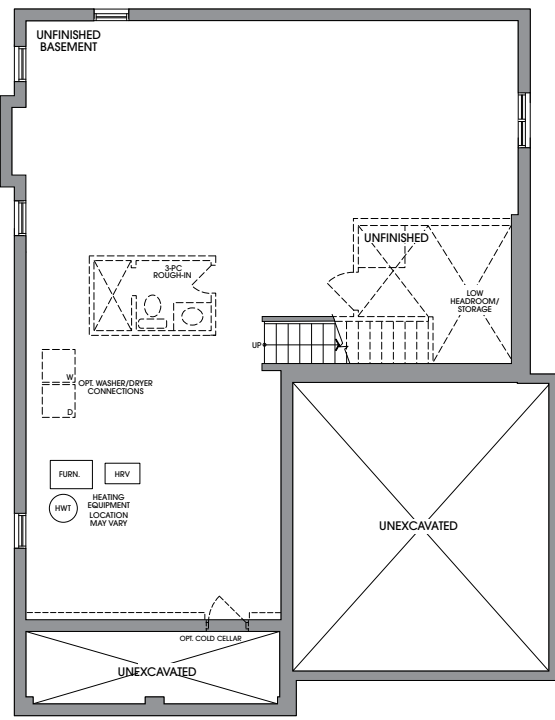
BASEMENT ELEVATION A, B & C
