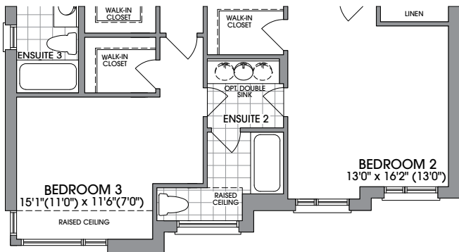
UPPER LEVEL ELEVATION C
