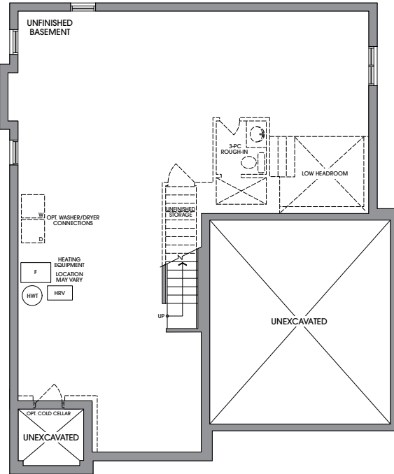
BASEMENT ELEVATION A
