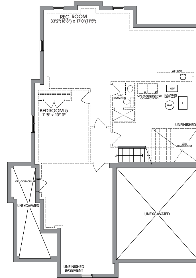
OPT. FINISHED BASEMENT ELEVATION A
