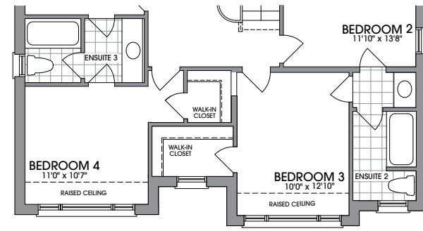
UPPER LEVEL ELEVATION C
