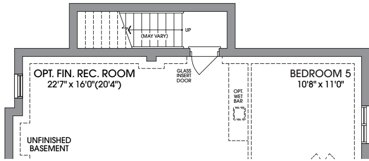
OPT. BASEMENT WALK-UP UNFINISHED & FINISHED BASEMENTS
