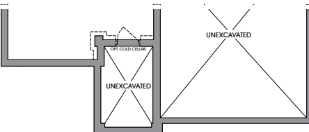
BASEMENT & OPT. FINISHED BASEMENT ELEVATION C
