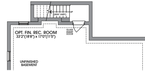
OPT. BASEMENT WALK-UP UNFINISHED & FINISHED BASEMENTS ELEVATION A & C
