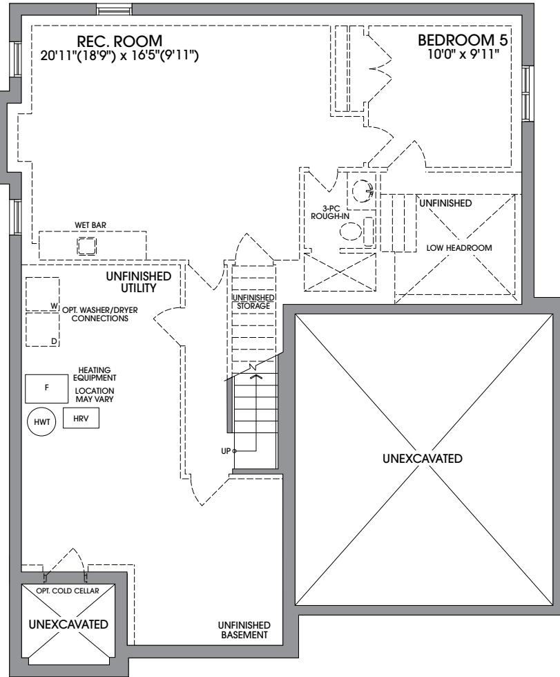
OPT. FINISHED BASEMENT ELEVATION A
