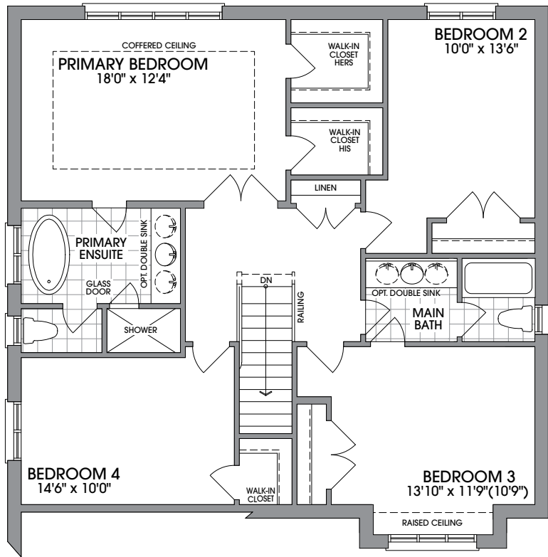
UPPER LEVEL ELEVATION A
