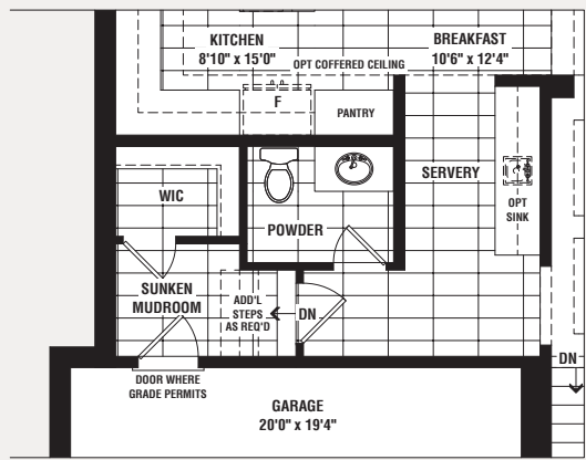
PARTIAL ALT MAIN FLOOR ELEV A' B' & C' W/ SERVERY
