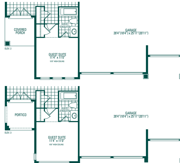
GUEST SUITE MAIN LEVEL
