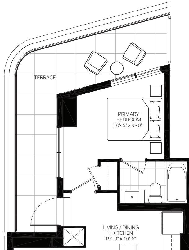
TERRACE CONDITION ON LEVEL 13
