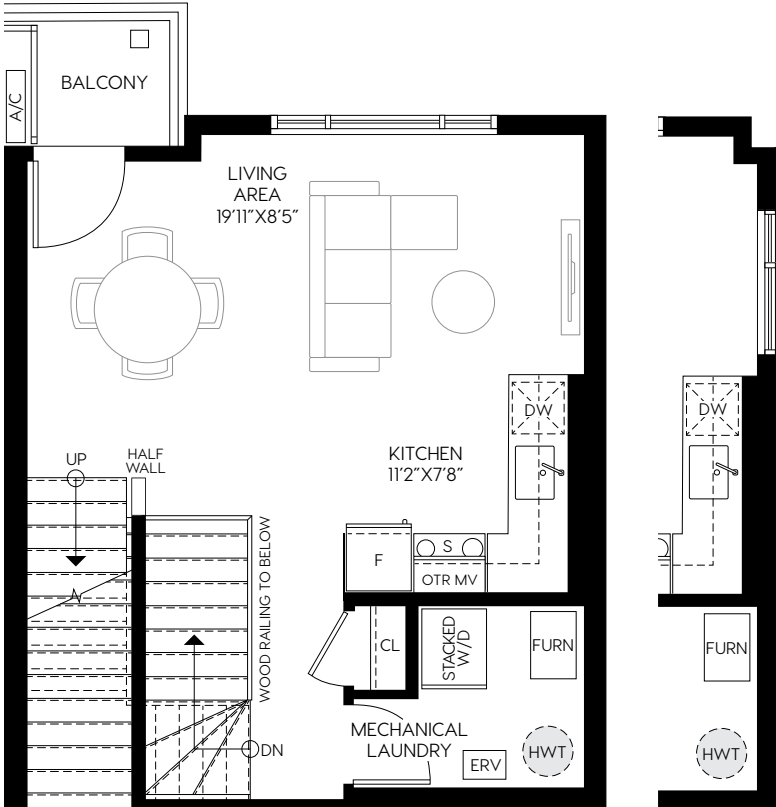
SECOND FLOOR INTERIOR UNITS 14, 16
