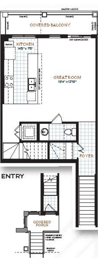
MAIN FLOOR
