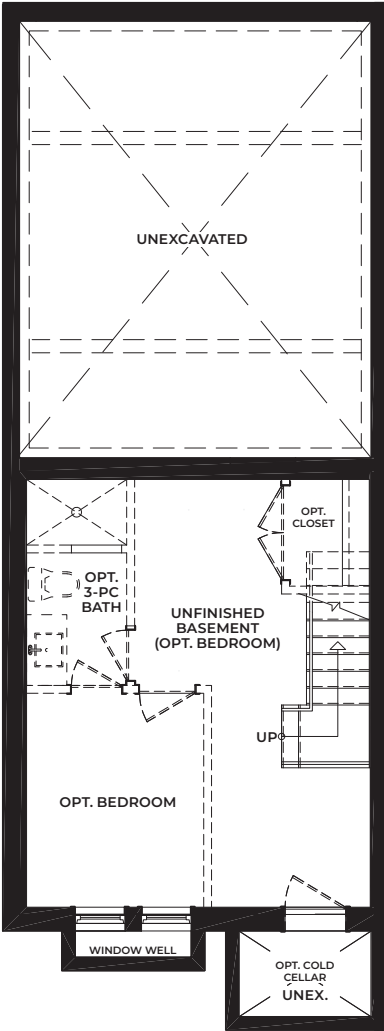
B1 End Opt. Bedroom BASEMENT
