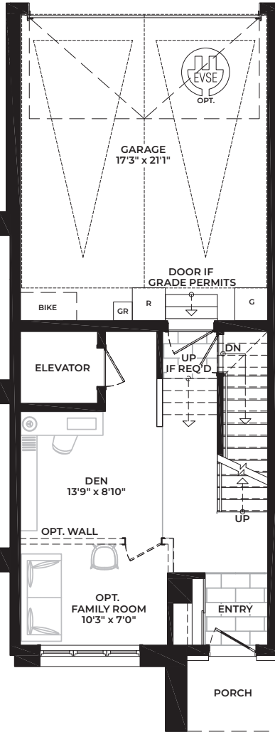
B1 End Opt. Elevator GROUND FLOOR
