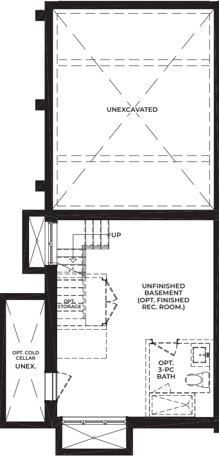
C1 Corner End BASEMENT
