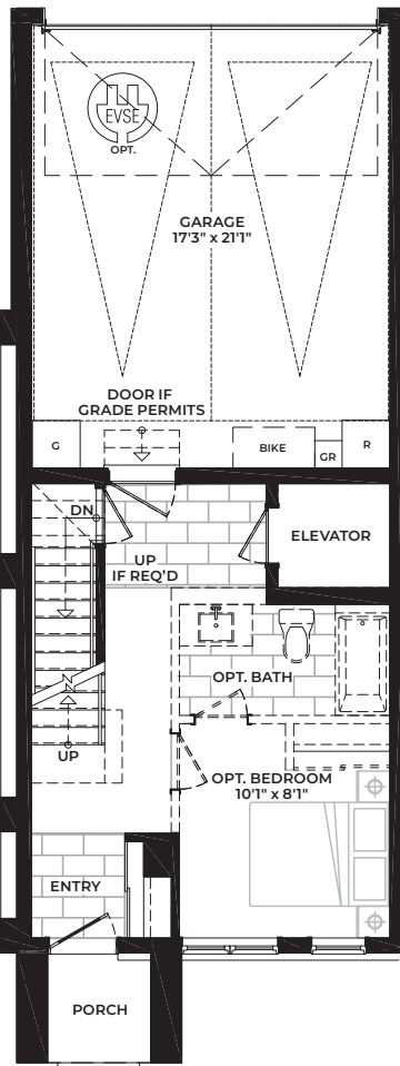
B1 B Porch End. Opt. Elevator & Opt. Bedroom GROUND FLOOR
