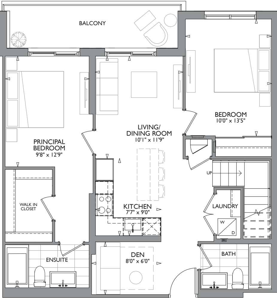
6TH FLOOR PLAN
