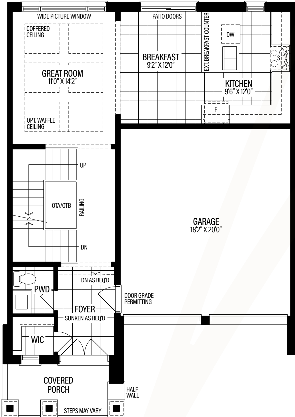
Main level ELEV 'A'
