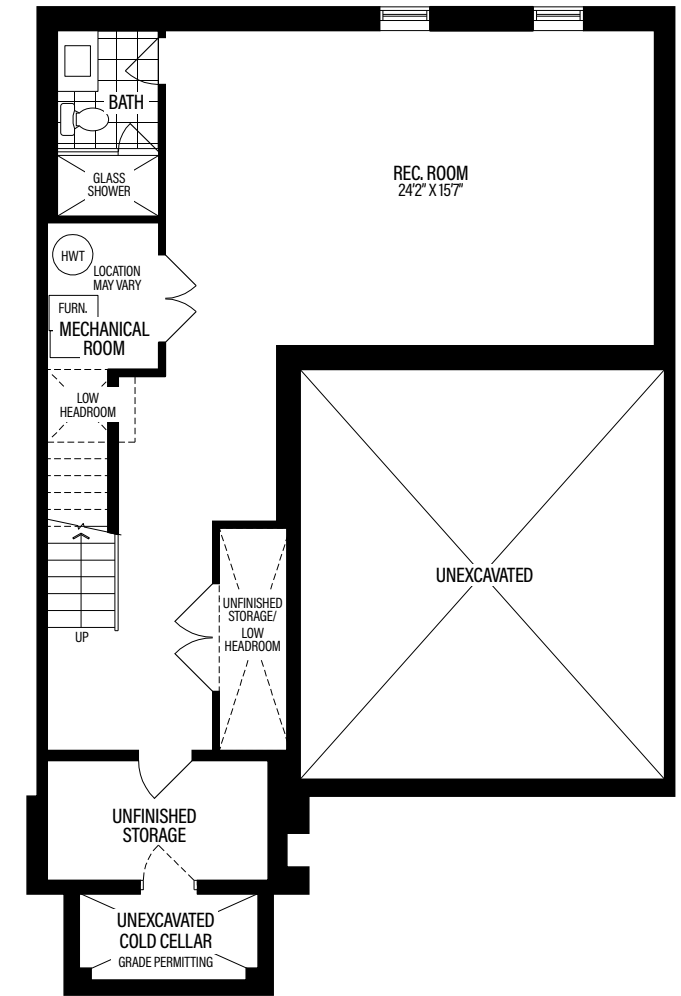
Lower Level ELEV 'A'
