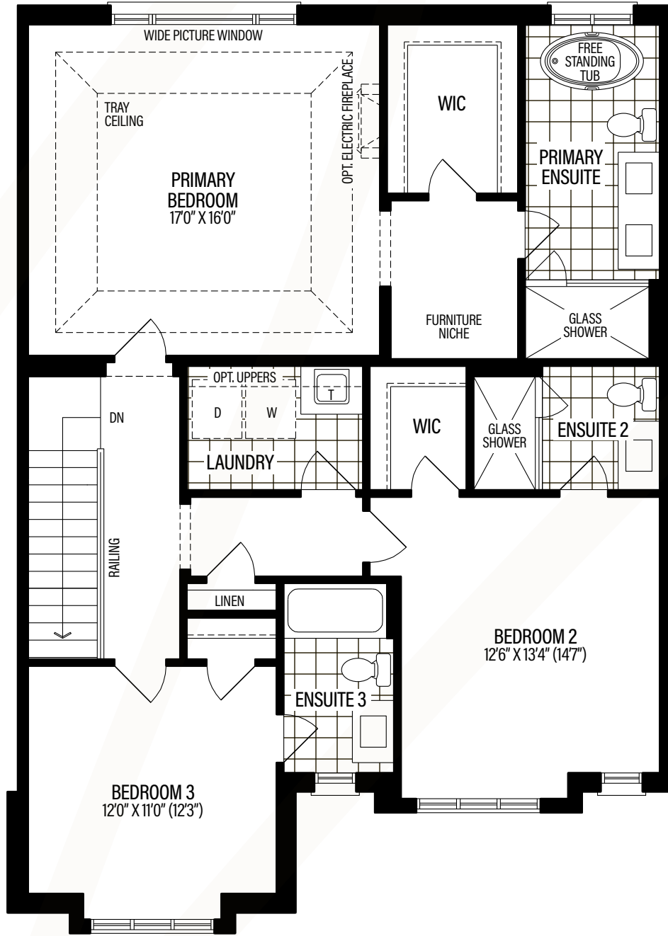
Second Level ELEV 'A'
