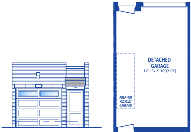
GARAGE ELEV.
