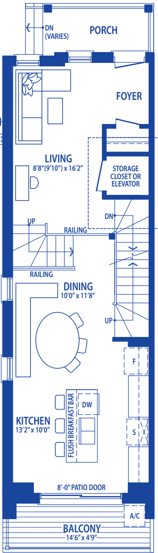
GROUND LEVEL
