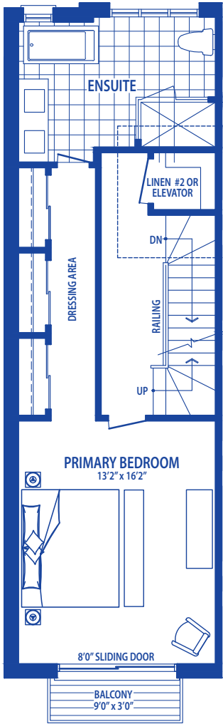
THIRD LEVEL
