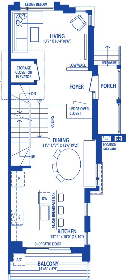
GROUND LEVEL
