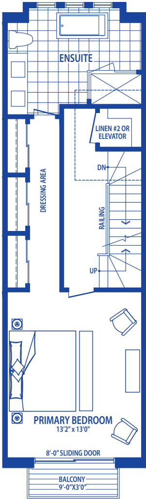
THIRD LEVEL
