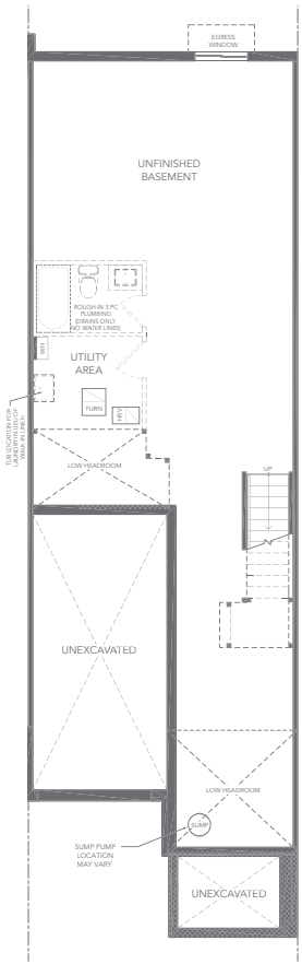
Basement - Elevation G
