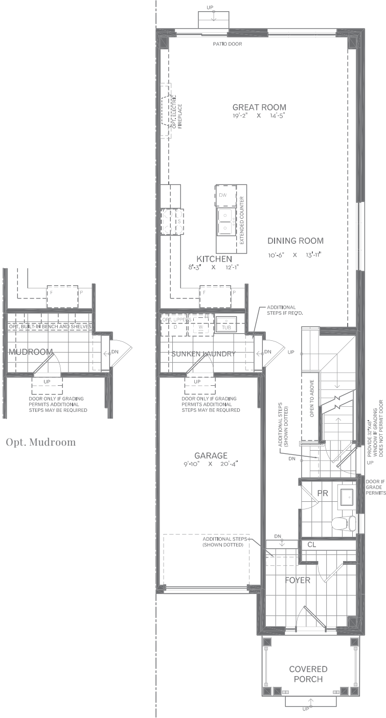
Ground Floor - Elevation D
