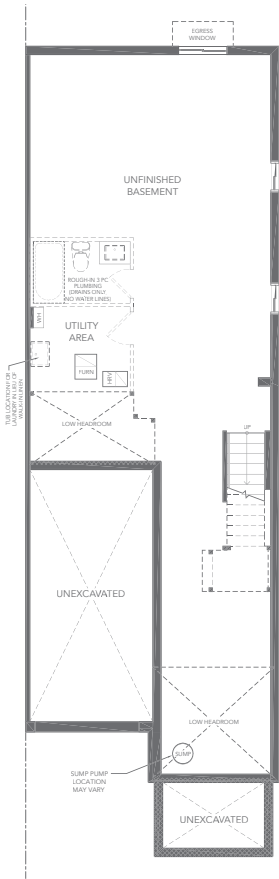
Basement - Elevation J
