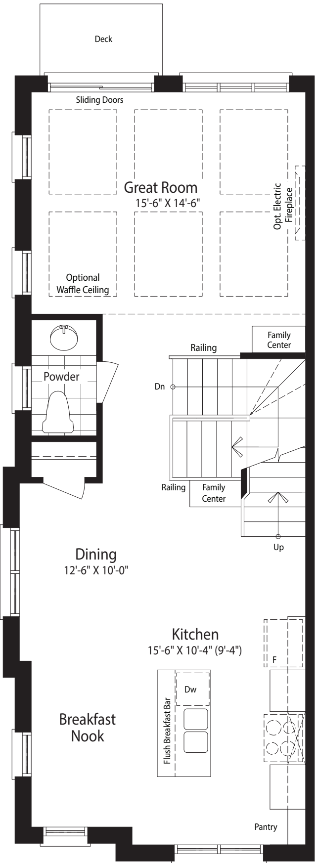
Alt. Main Floor Plan Elevation 'A1'
