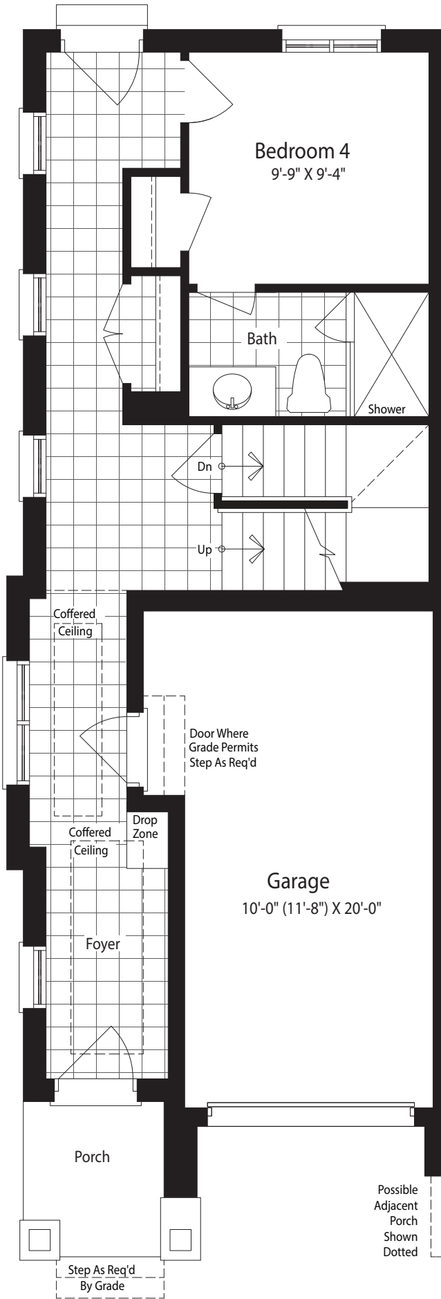
Ground Floor Plan - Elevation 'A1' & 'A2'
