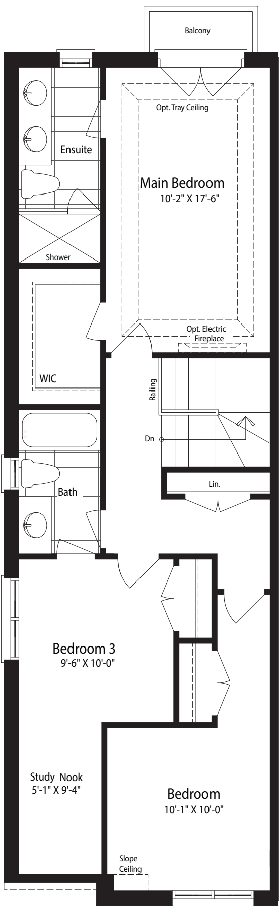
Upper Floor Plan Elevation 'A1'
