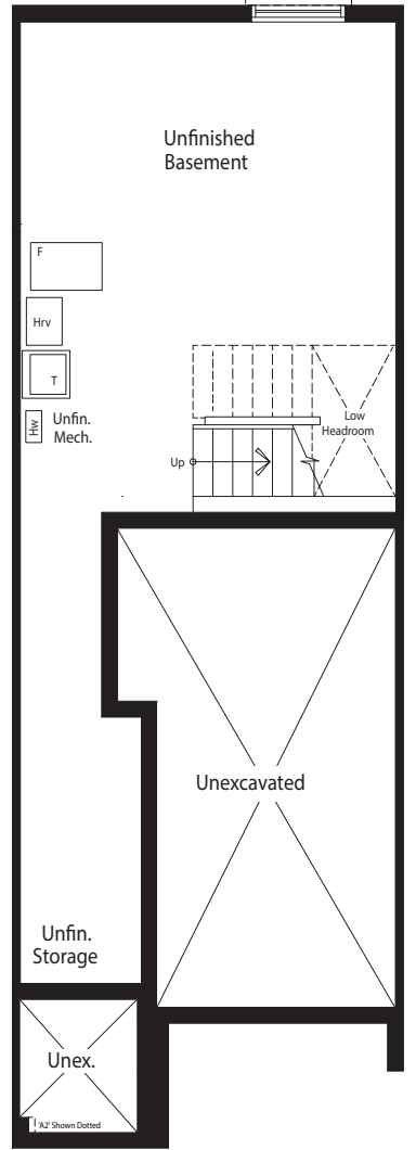
Lower Floor Plan Elevations 'A1' & 'A2'
