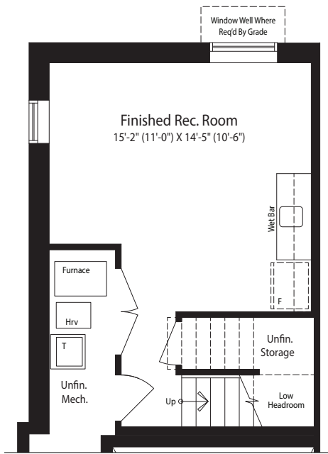
Opt. Finished Lower Floor Plan Elevation 'A1', 'A2', 'B1' & 'B2' Only available at time of decor appointment
