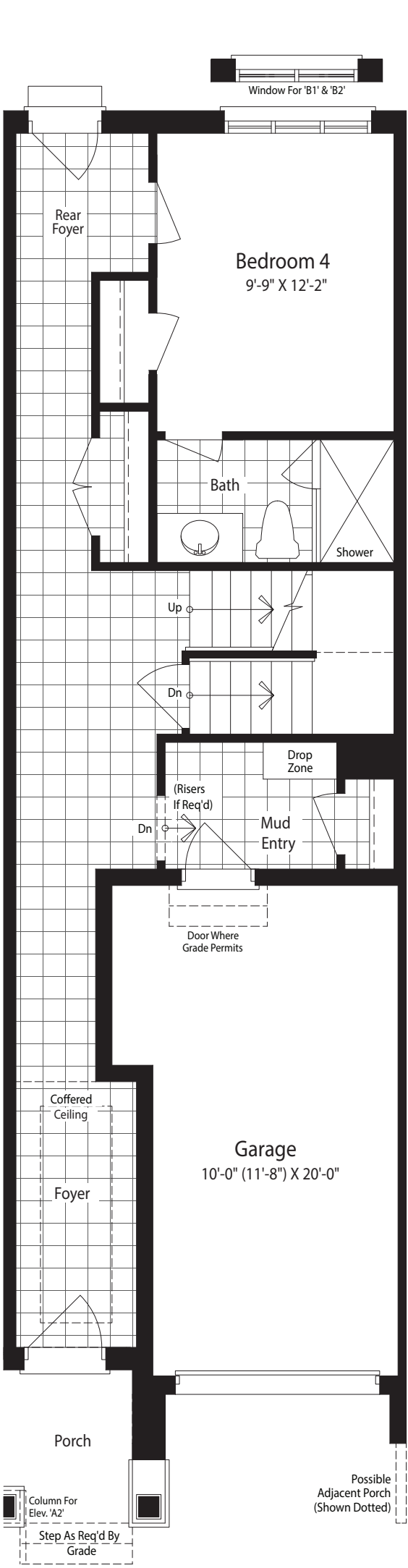
Ground Floor Plan - Elevation 'A1' & 'A2'
