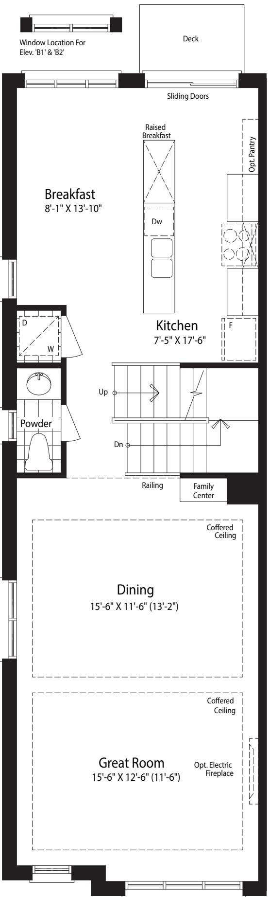
Alt. Main Floor Plan Elevation 'A1'
