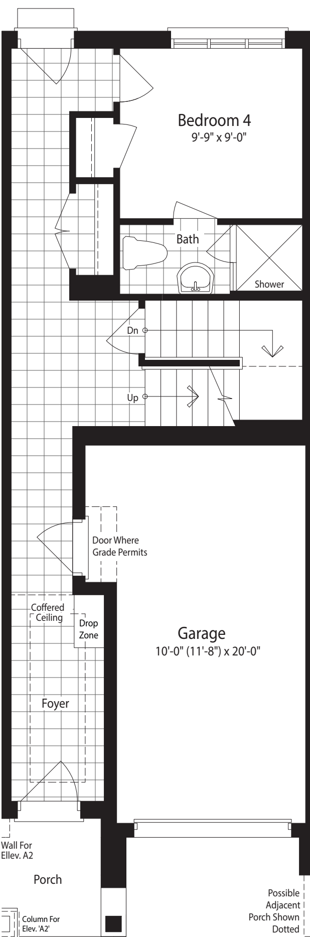
Ground Floor Plan Elevation 'A1' & 'A2'
