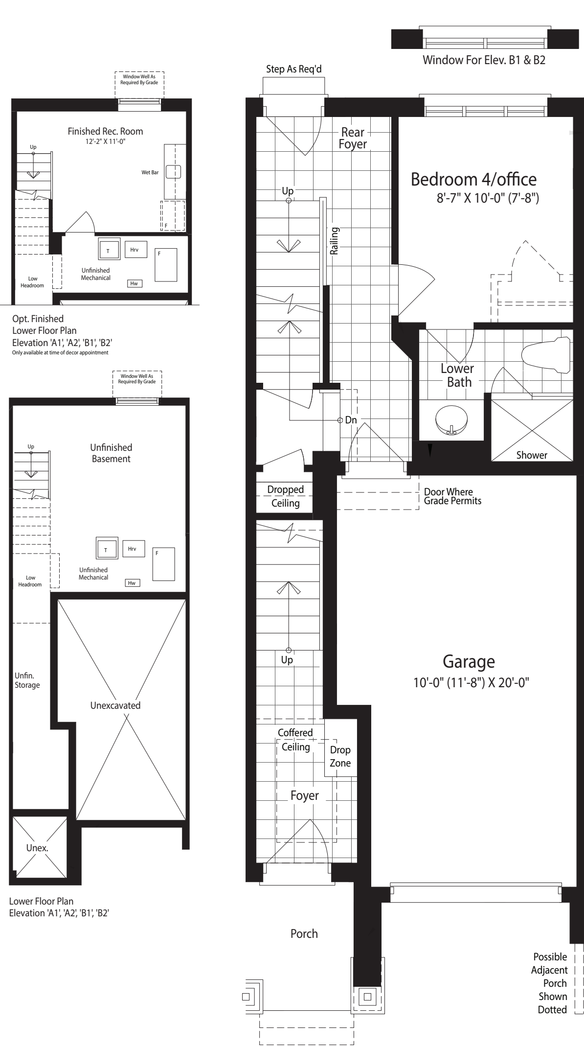
Ground Floor Plan Elevation 'A1'
