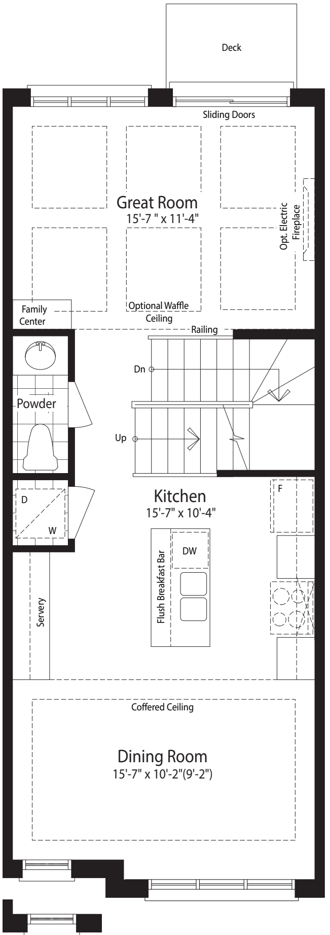
Main Floor Plan Elevation 'A1' & 'A2'
