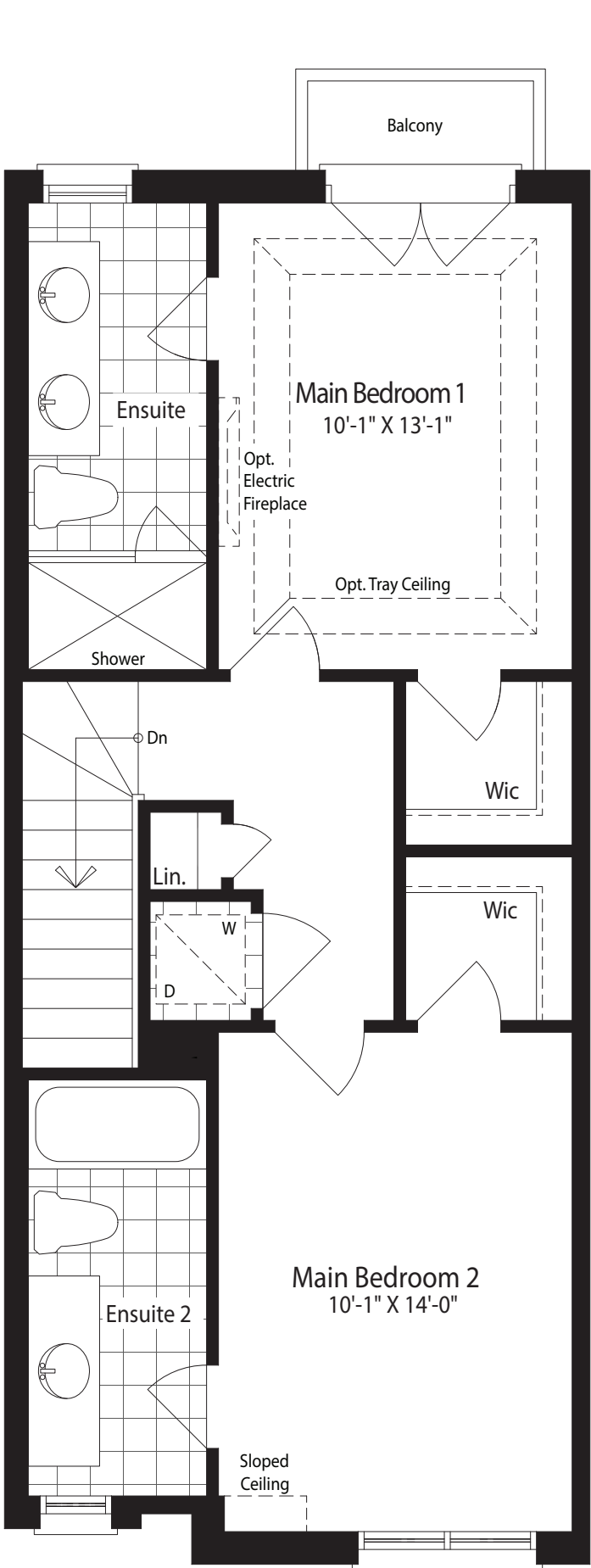
Upper Floor Plan Elevation 'A1'
