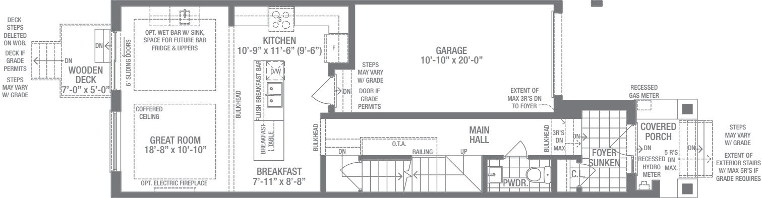
GROUND LEVEL
