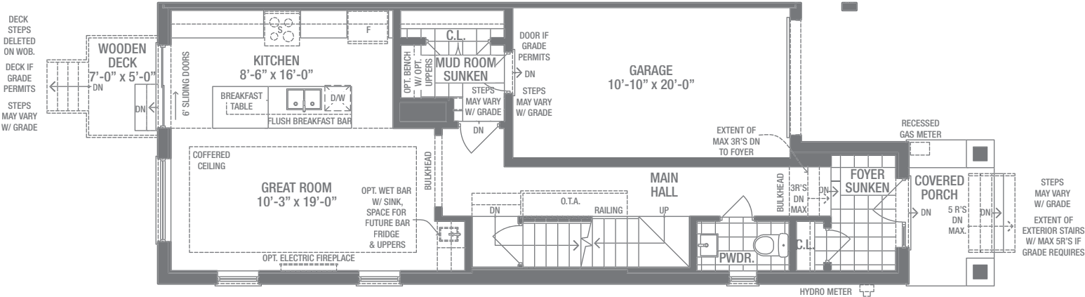
GROUND LEVEL
