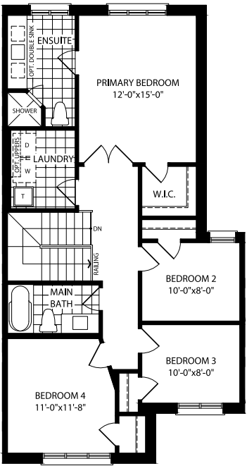
OPTIONAL SECOND FLOOR A 4 BEDROOM
