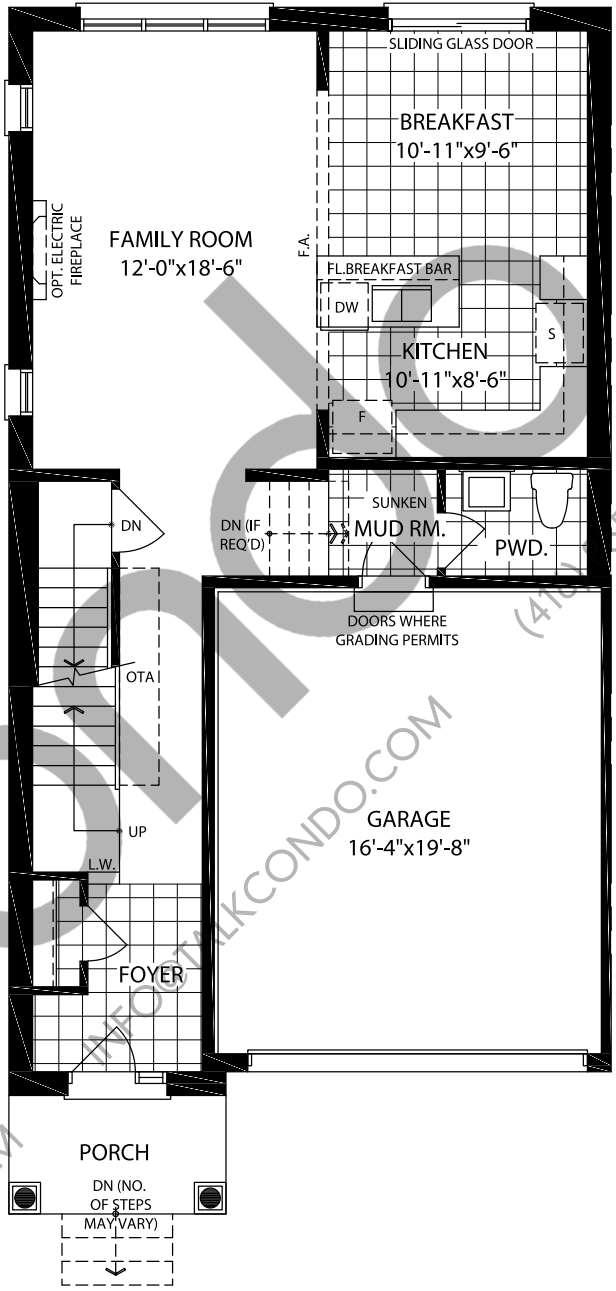
MAIN FLOOR A
