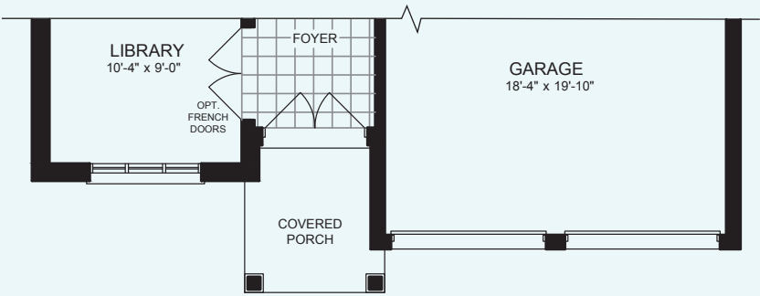
PARTIAL GROUND FLOOR PLAN ELEVATION B
