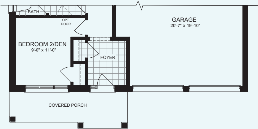
PARTIAL GROUND FLOOR PLAN ELEVATION B
