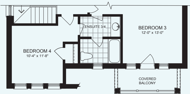
PARTIAL SECOND FLOOR PLAN ELEVATION B
