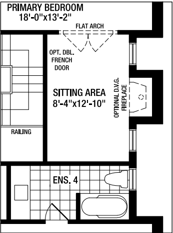
PARTIAL OPTIONAL PRIMARY SITTING AREA FOR 4 BED PLAN
