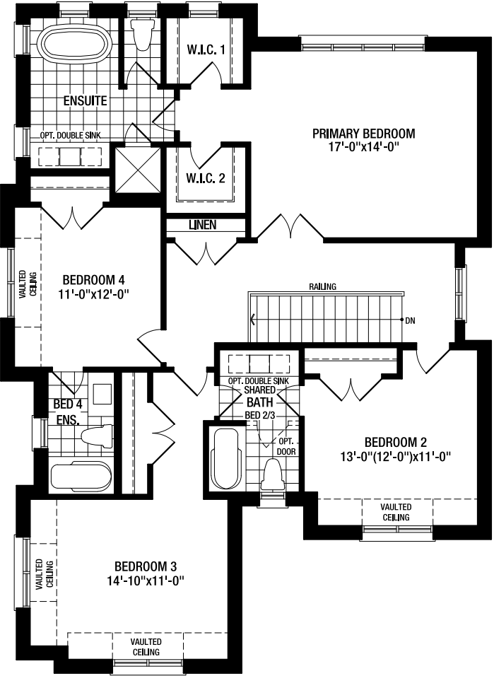
SECOND FLOOR A
