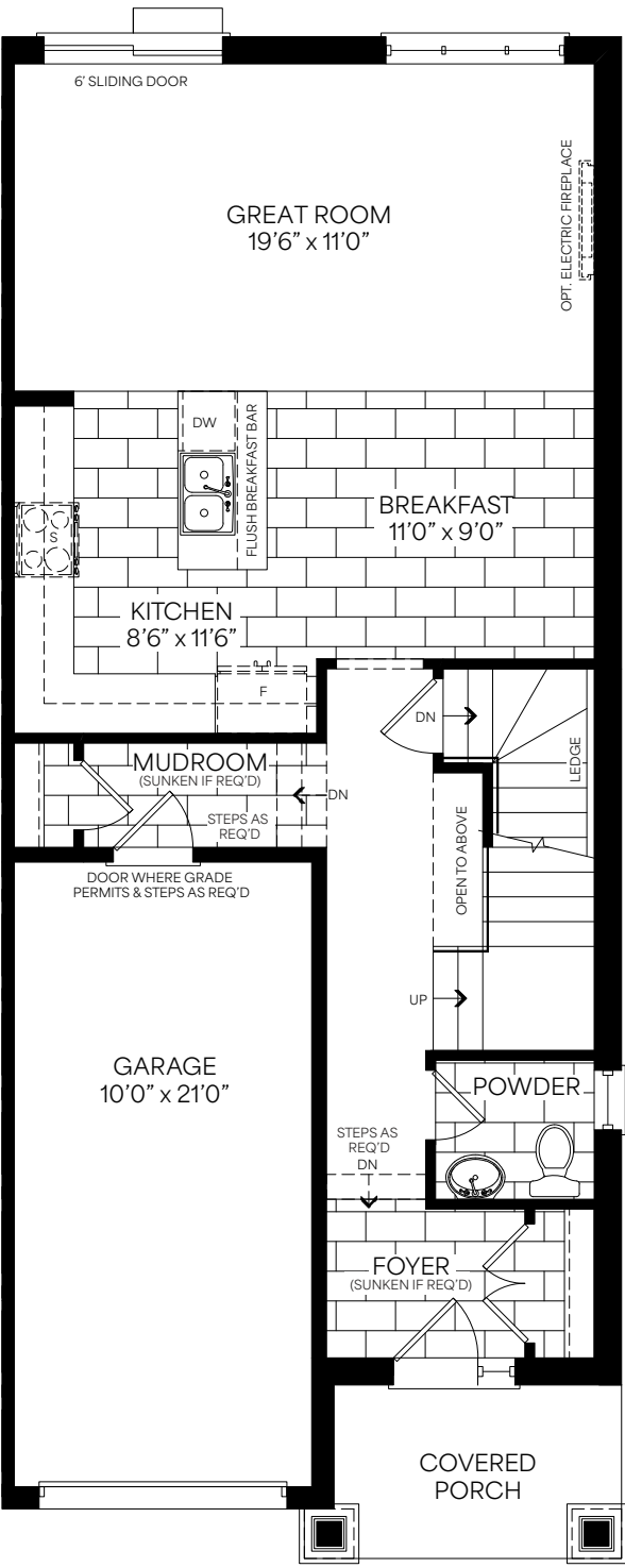
Main Floor Elevation A1 & A2
