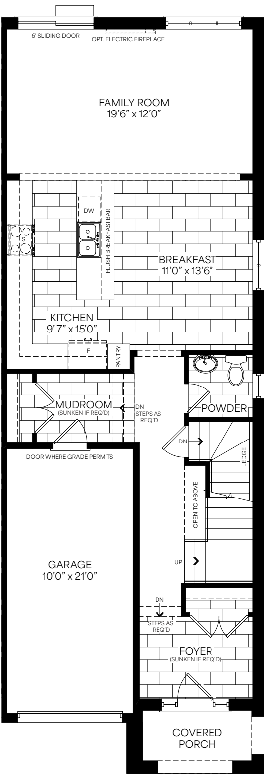
Main Floor Elevation A1 & A2
