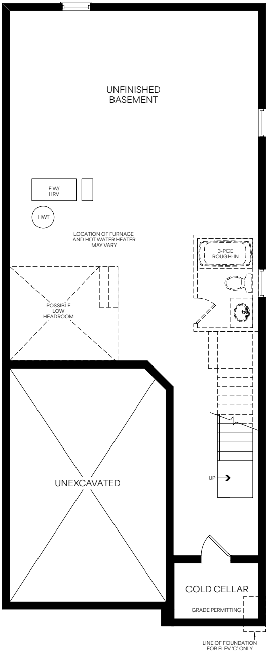
Basement Elevation A, B, C, & D
