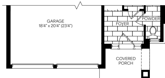
Main Floor Elevation C
