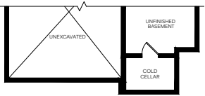
Basement Elevation B
