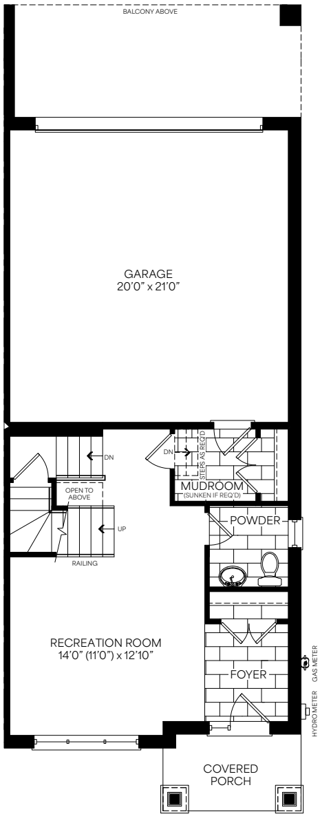
Ground Floor Elevation A
