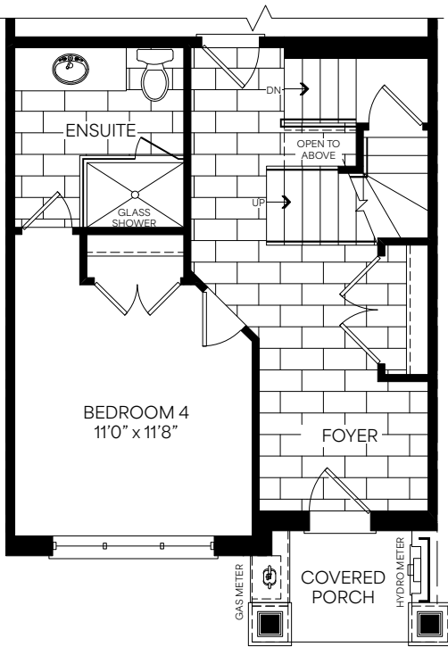
Opt. Ground Floor 4 Bedroom Elevation A
