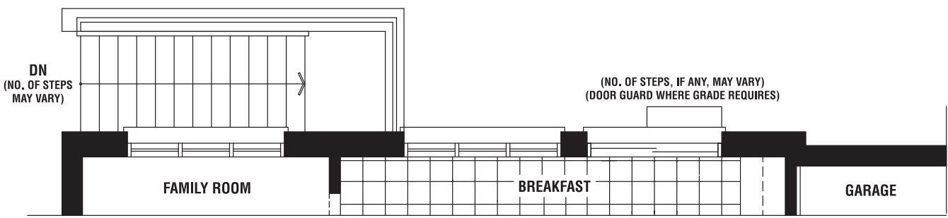
PARTIAL GROUND FLOOR PLAN OPT. WALK UP BASEMENT CONDITION (SUBJECT TO GRADING APPROVAL) (LOCATION MAY VARY)
