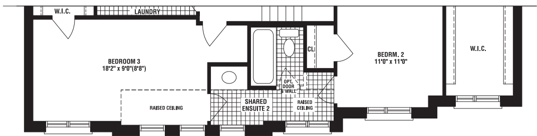
PARTIAL SECOND FLOOR PLAN ELEV. 'C'
