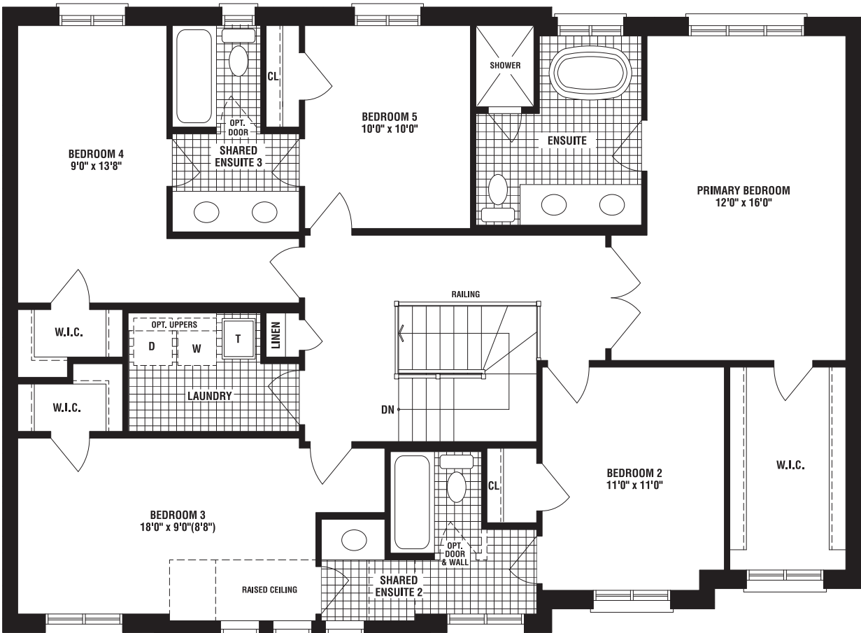
SECOND FLOOR PLAN ELEV. 'A'
