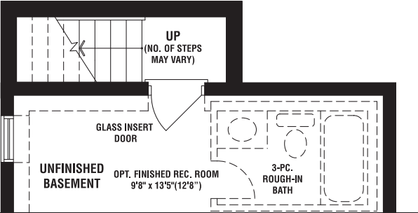
PARTIAL BASEMENT PLAN WALK-UP CONDITION (SUBJECT TO GRADING APPROVAL)
