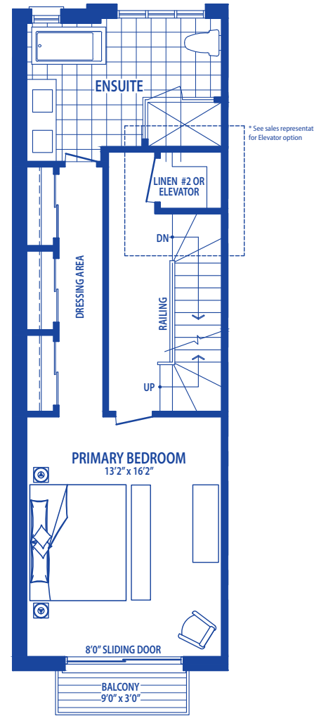
THIRD LEVEL
