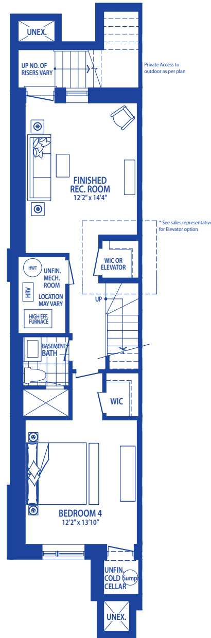
BASEMENT
