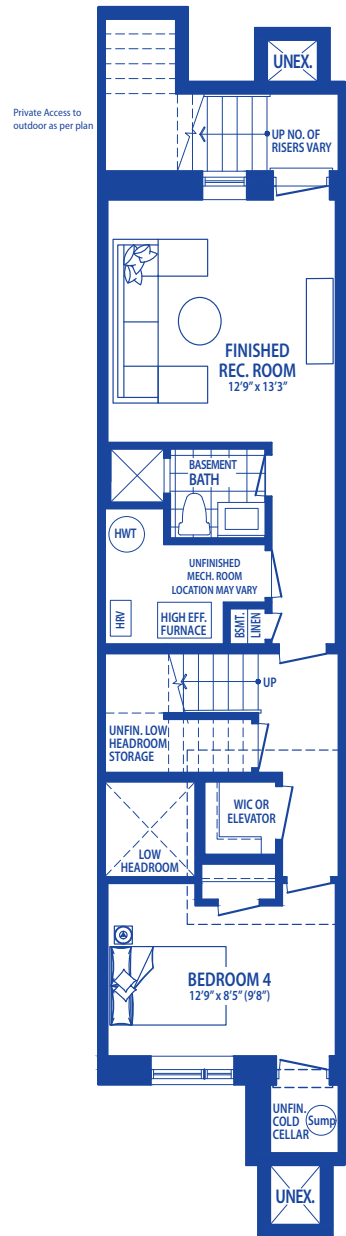
BASEMENT
