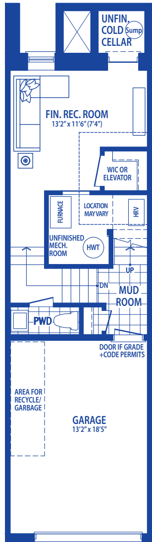
BASEMENT
