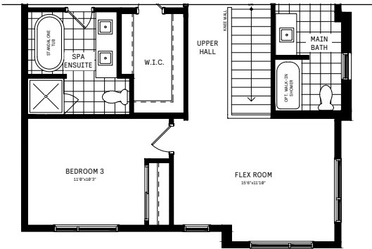
8 Spa Ensuite w/ Flex Room
