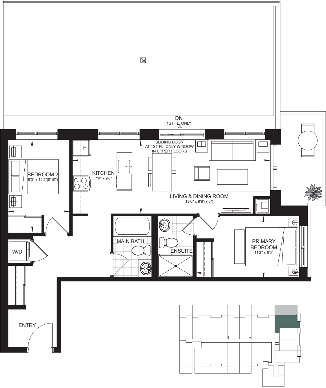
1ST FLOOR
