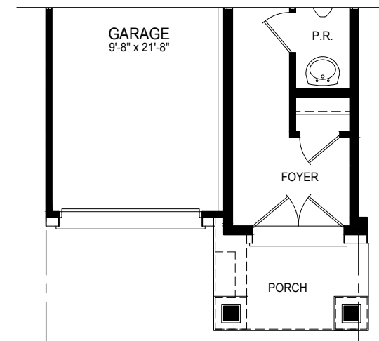
Ground Level Elev. A2
