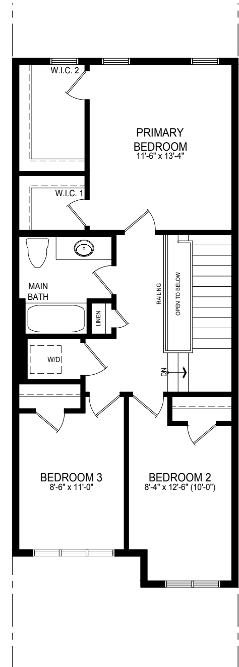
Upper Level Floor Elev. A1
