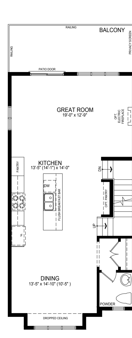
Main Floor Elev. A1
