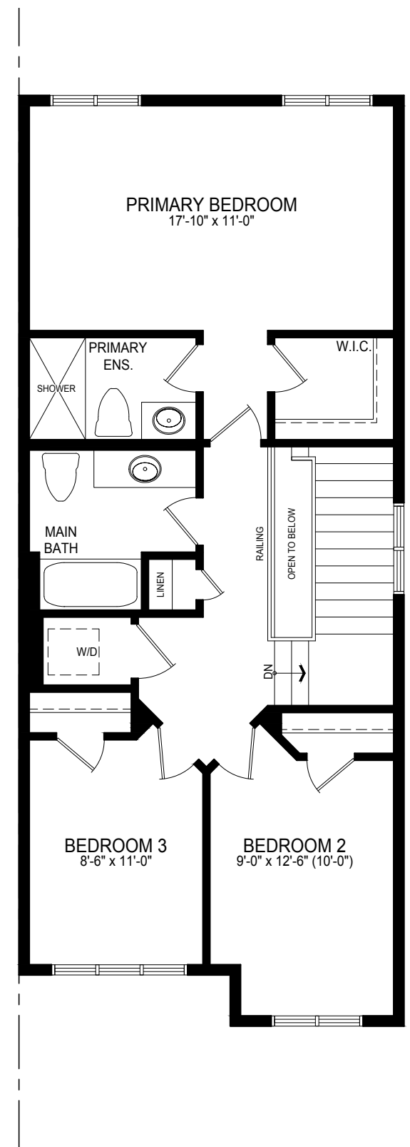
Upper Level Floor Elev. A1
